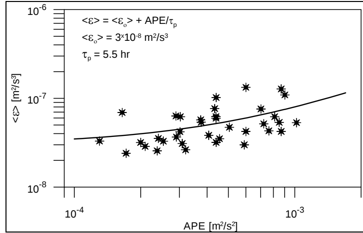
Fig. 5. The averaged dissipation rate in the pycnocline of SCS as a function of available potential energy; \tau_p is a characteristic dissipation time of APE.
