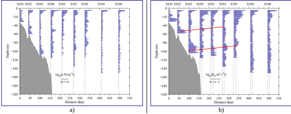
Fig.3. The dissipation rate \varepsilon(z) (left) and the diffusivity K_N(z) (right) profiles, respectively, along the section S highlighted in Fig. 2. The red lines in b) indicate enhanced mixing along a possible ray of internal waves reflected from the shelf break [Lien and Gregg 2001].
