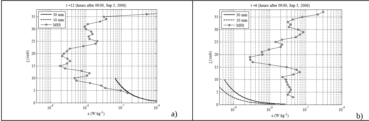
Fig. 6. The MMS dissipation profiles \epsilon_{mc}(\zeta) and the law-of-the-wall profiles \epsilon_b(\zeta) for the across-slope eastern (a) and western (b) flow ( \tau_{avr} = 30 and 10 min).
