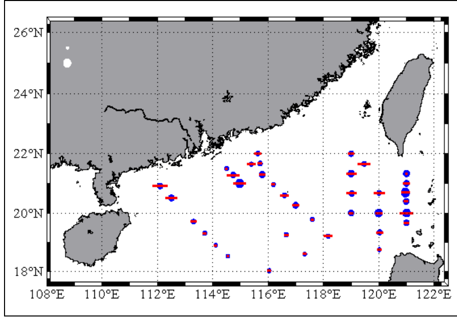
Fig. 4. The averaged dissipation rate \langle \varepsilon_p \rangle (blue circles) and the estimates of APE of internal waves per unit mass (red horizontal bars) in the upper pycnocline of SCS. The dissipation rate is scaled between 2.4 \times 10^{-8} and 1.3 \times 10^{-7} \text{ m}^2/\text{s}^3 and APE is between 1.3 \times 10^{-4} and 10^{-3} \text{ m}^2/\text{s}^2 .
