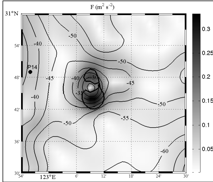
Fig. 7. Local bathymetry and the internal tide generating body force F near and to the east of the point of measurements (P14); F > 0.25 \text{ m}^2/\text{s}^2 is encircles the small seamount.
