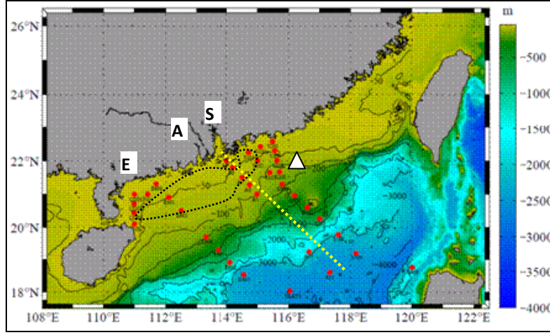
Fig.2. Stations of the XMU cruise taken in SCS in July 2009. Three longest across shelf sections are marked E, A, and S, and the triangle is the measurement site of St Laurent [2008].
