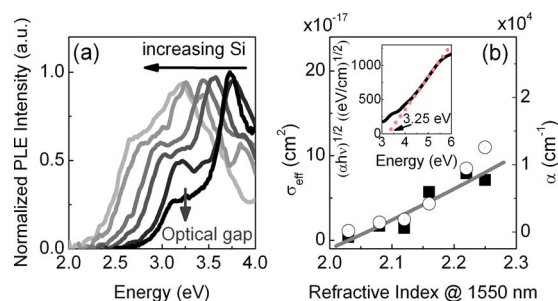
FIG. 2. (Color online) (a) Normalized PLE spectra collected at 1.54 microns from Er:SiN x samples with various excess Si at. %. (b) The effective excitation cross sections \sigma_{eff} (squares) and the absorption coefficients \alpha at 458 nm (circles) of the Er:SiN x samples with different excess Si at. %. The straight line is to guide the eye. In the inset: The optical gap calculated from the Tauc plot of the stoichiometric sample which is highlighted with an arrow in (a).
