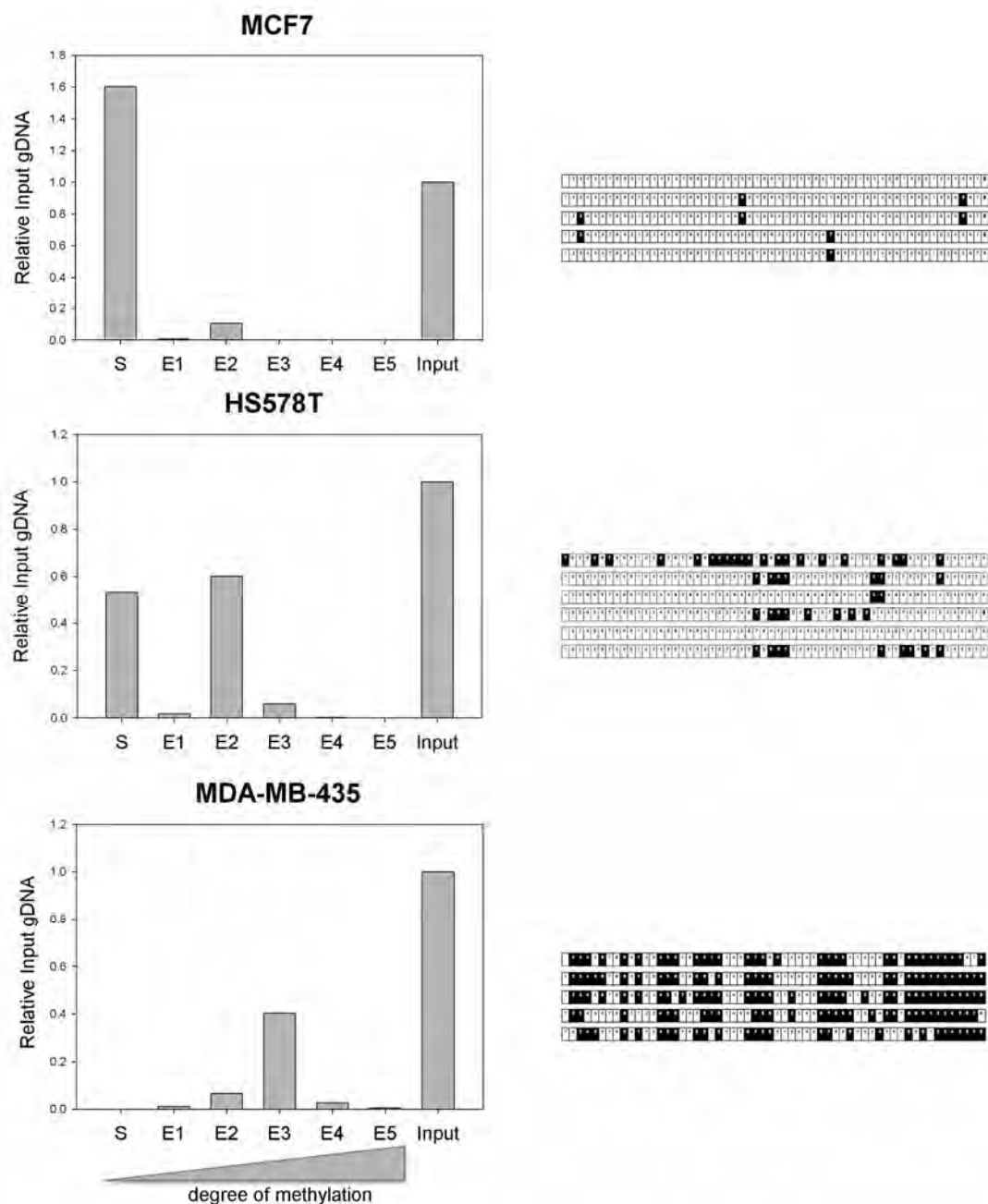
Figure 4. The MethyMiner assay correlates directly with promoter methylation analysis for PHD3. DNA extracted from the respective cell lines was tested using the assay outlined in Figure 3. After elution of DNA, quantitative real-time PCR analysis of the PHD3 promoter was performed to assess the methylation status within these cells. Results demonstrated that the low PHD3 expressing cell line (MDA-MB-435) had higher methylation, and this correlated with the DNA methylation analysis from our last report (right panel – Black squares indicate methylated CpG, White squares indicate Unmethylated CpG). The opposite was true of the high PHD3 expressing cell line MCF7, and intermediate results were found with the partial-expressing cell line HS578T.
