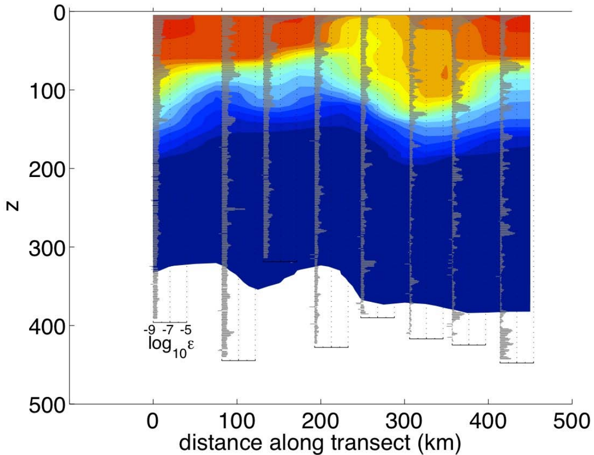
Figure 3: Temperature and turbulent dissipation rate ( \epsilon ) across the region of the cold wake for section 1, at t=3 days after the passage of the typhoon. Distance along the transect runs from south to north. Temperature contours are from 15 to 30 C, and the cold wake signal is clearly visible between the 200 to 400 km section of the transect
