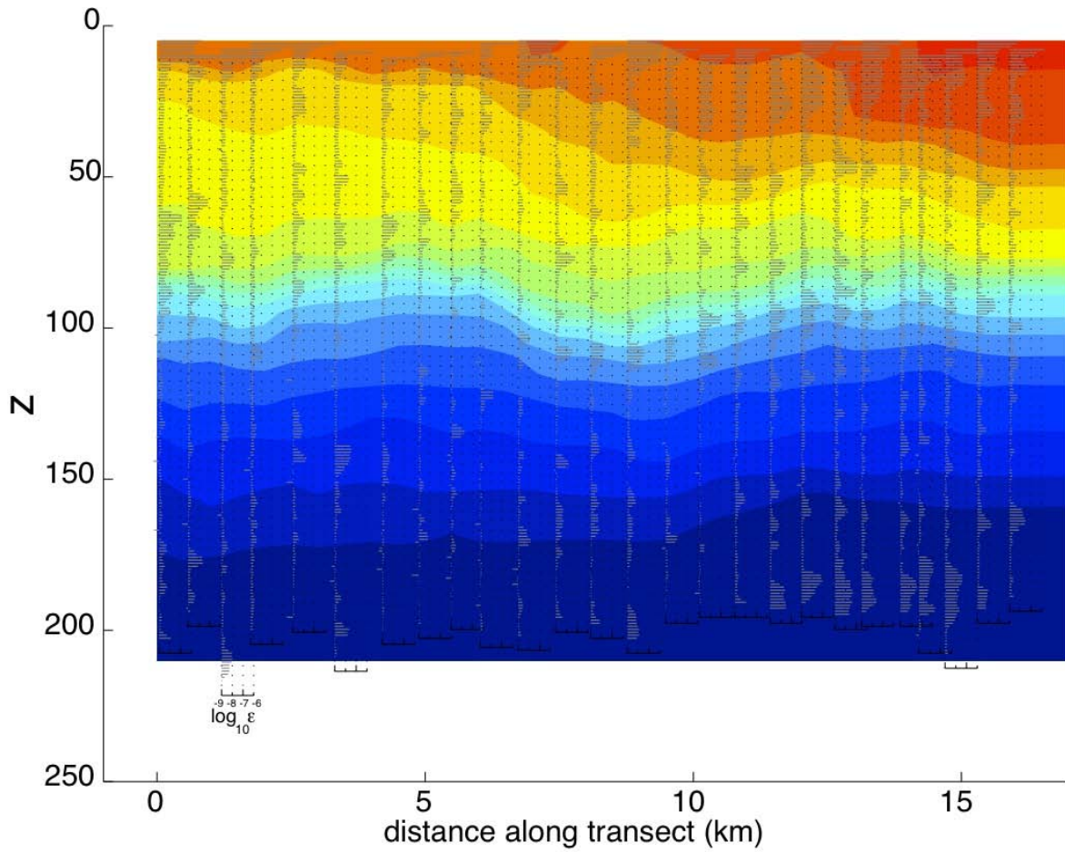
Figure 5: Temperature and turbulent dissipation rate ( \varepsilon ) across the region of the cold wake for section 3, at t=4 days after the passage of the typhoon. Distance along the transect runs from south to north. Temperature contours are from 15 to 30 C. This section runs from inside the wake through the north edge into the background stratification.
