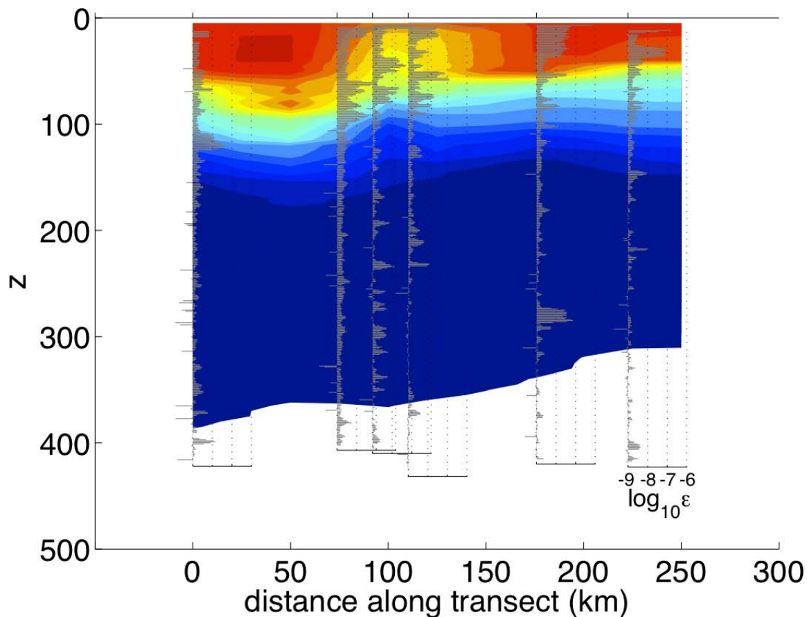
Figure 4: Temperature and turbulent dissipation rate ( \epsilon ) across the region of the cold wake for section 2, at t=3.5 days after the passage of the typhoon. Distance along the transect runs from south to north. Temperature contours are from 15 to 30 C, and the cold wake signal is clearly visible between the 50 to 150 km section of the transect.
