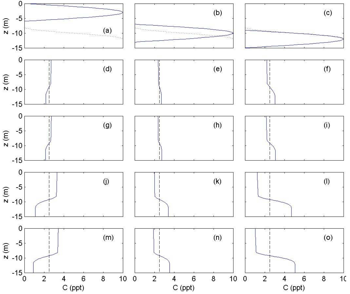
Figure 5: Concentration profiles for a passive scalar C in a two-layered stratified tidally-driven channel flow. Subplots (a) – (c) show the initial distribution of the passive scalar plume. Final concentrations profiles are shown in subplots (d) - (f) using the Peters et al. model; subplots (g) - (i) using the Munk and Anderson model; subplots (j) - (l) using the Venayagamoorthy and Stretch model; subplots (m) - (o) using the Kim and Mahrt model, respectively. Also superimposed on subplots (d) – (o) are the final profile for the unstratified case profile (from Elliott and Venayagamoorthy 2010).
