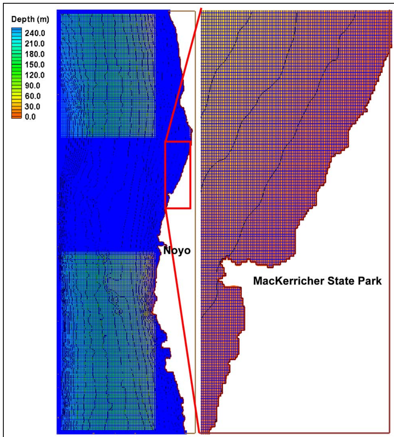
Figure 1. CMS domain, grid, and bathymetry.
