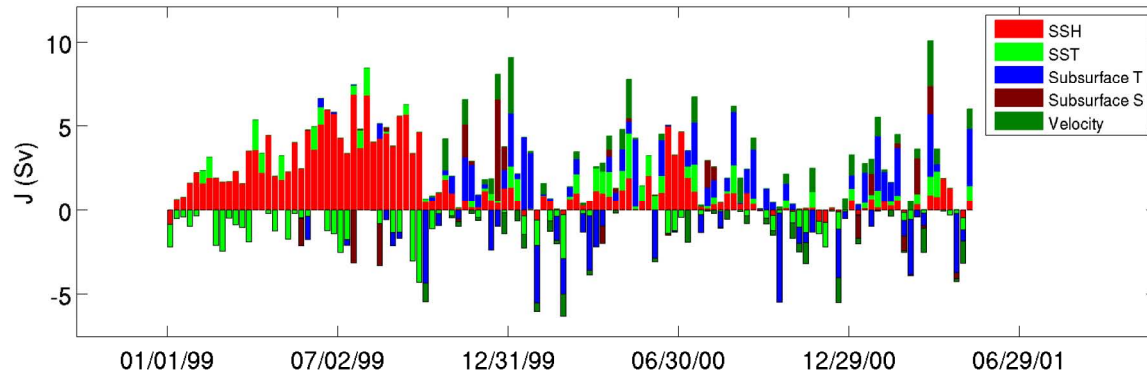
Figure 1: A time series of the Yucatan transport increment (i.e. posterior transport minus prior transport) for each 4D-Var assimilation cycle. The contribution of each observing platform to the transport increment is indicated by the different colored bars, while the sum of all the bars represents the total transport increment.
