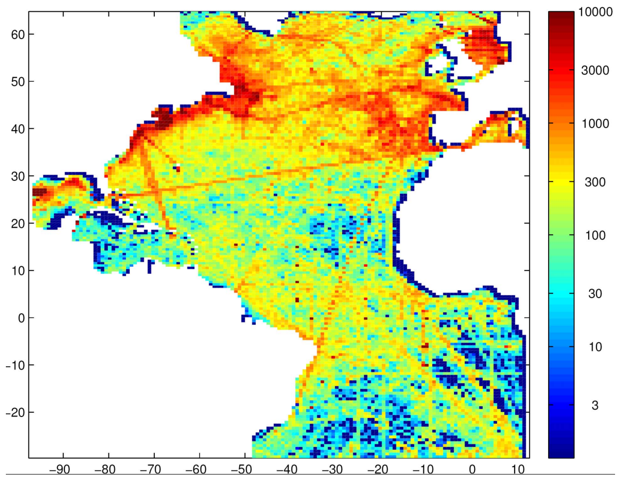
Figure 4: The number of in situ hydrographic observations available during the period 1993-2005 that fall within each grid cell of the new ROMS ATL model domain.
