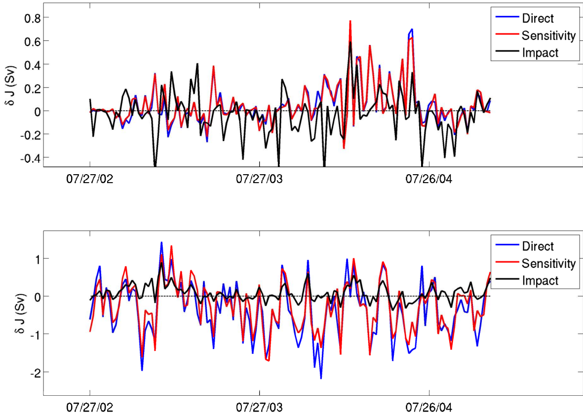
Figure 3: Time series (blue curves) of the change in 37N transport computed directly from the prior and posterior circulations estimates of each 7-day 4D-Var cycle when (a) all Argo observations are withheld, and (b) all satellite SSH observations are withheld. Also shown are time series (red curves) of the change in 37N transport based on the predictions of observation sensitivity analyses. Time series based on the predictions of observation impact analyses are shown by the black curve.
