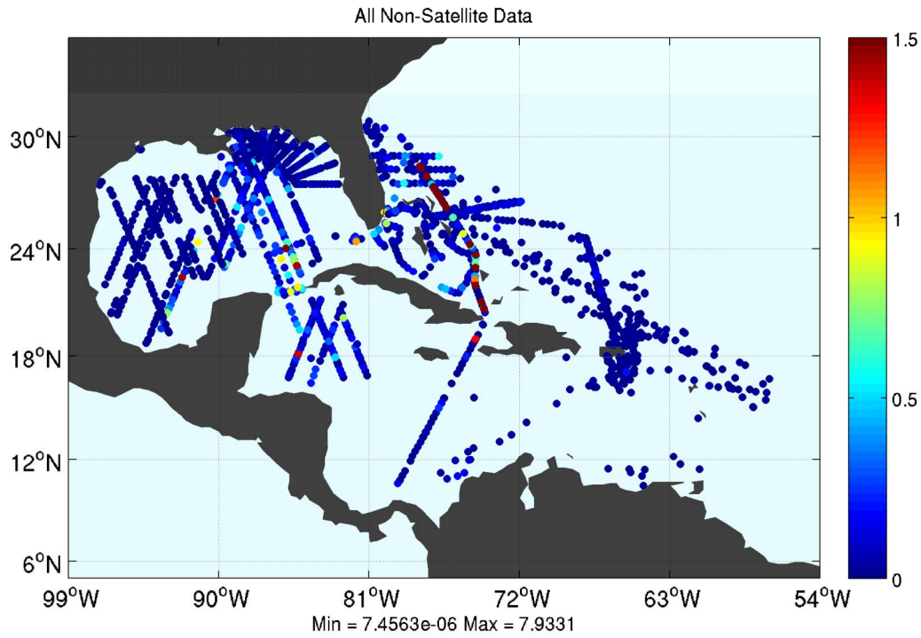
Figure 2: The rms impact of in situ observations on Yucatan transport increments averaged over all data assimilation cycles.
