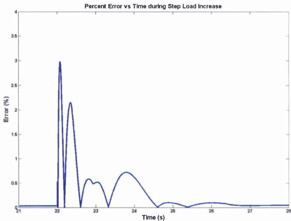
Figure 18: Error of machine speed when the rotational inertia of gas turbine emulator following a 20% increase of electric load
