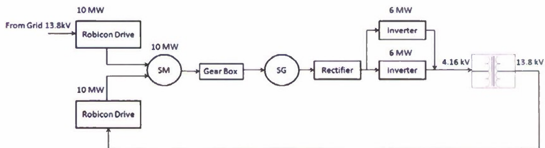
Figure 25. Configuration for re-circulating generated power
