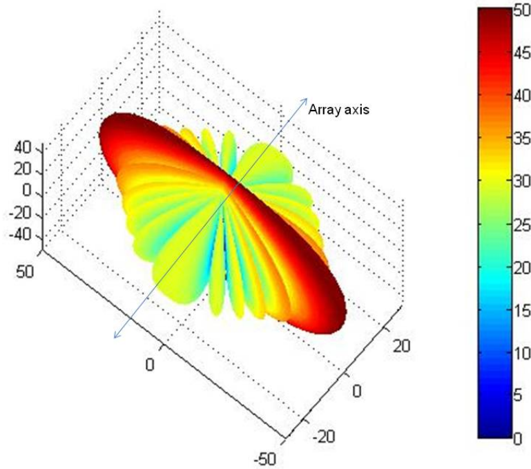
Figure 7 Three-Dimensional Linear Beampattern for a Pressure Sensor Array Due to Incoming Signal at Broadside
