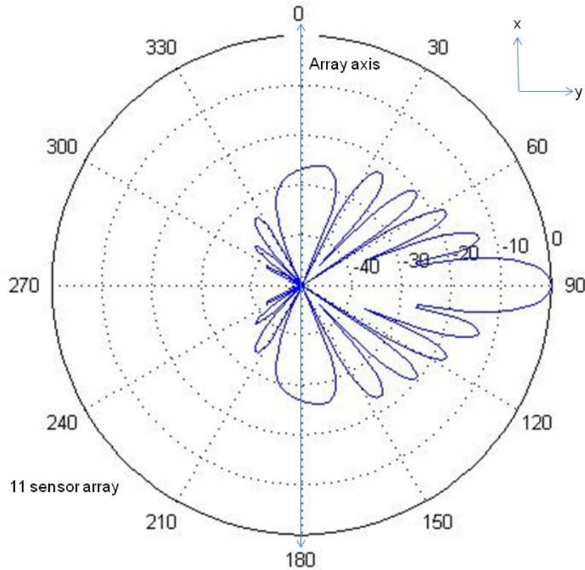
Figure 11 Cardioid Beampattern for a Vector Sensor Array Due to Incoming Signal at Broadside
