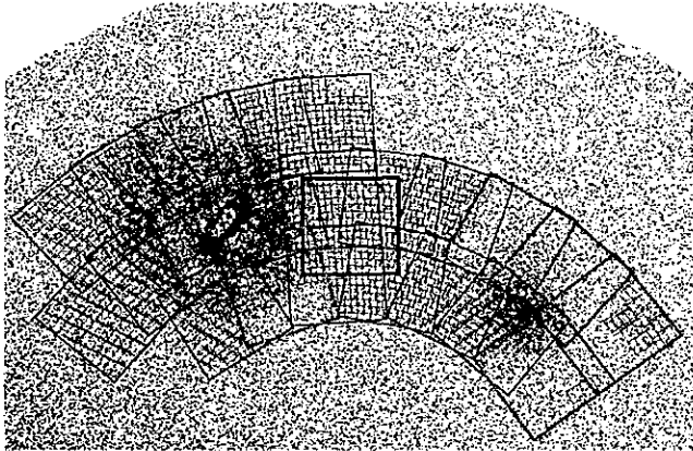
Figure 1. SPM fields in the Magellanic Cloud area. Gray outlined regions correspond to second-epoch SPM plate observations. The small squares indicate second-epoch CCD observations. The black outlined area is the VMC region (see Section 4.2). A subset of stars from the USNO-A2.0 Catalog is plotted in the background to indicate the positions of the LMC (on the left) and SMC (on the right). SPM fields are on nominal 5° centers, not including the VMC field.
