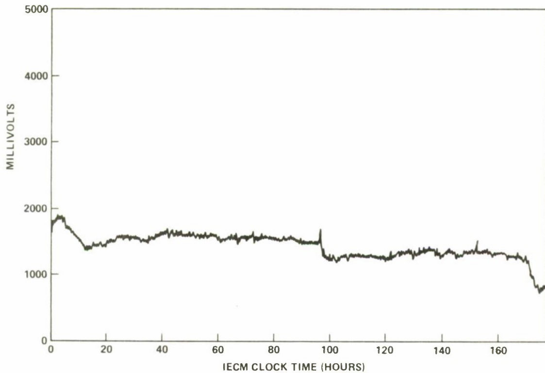
Figure IV-3. OEM-Spacelab 1 diffuse reflection signal channel I_3 - MgF_2 .
