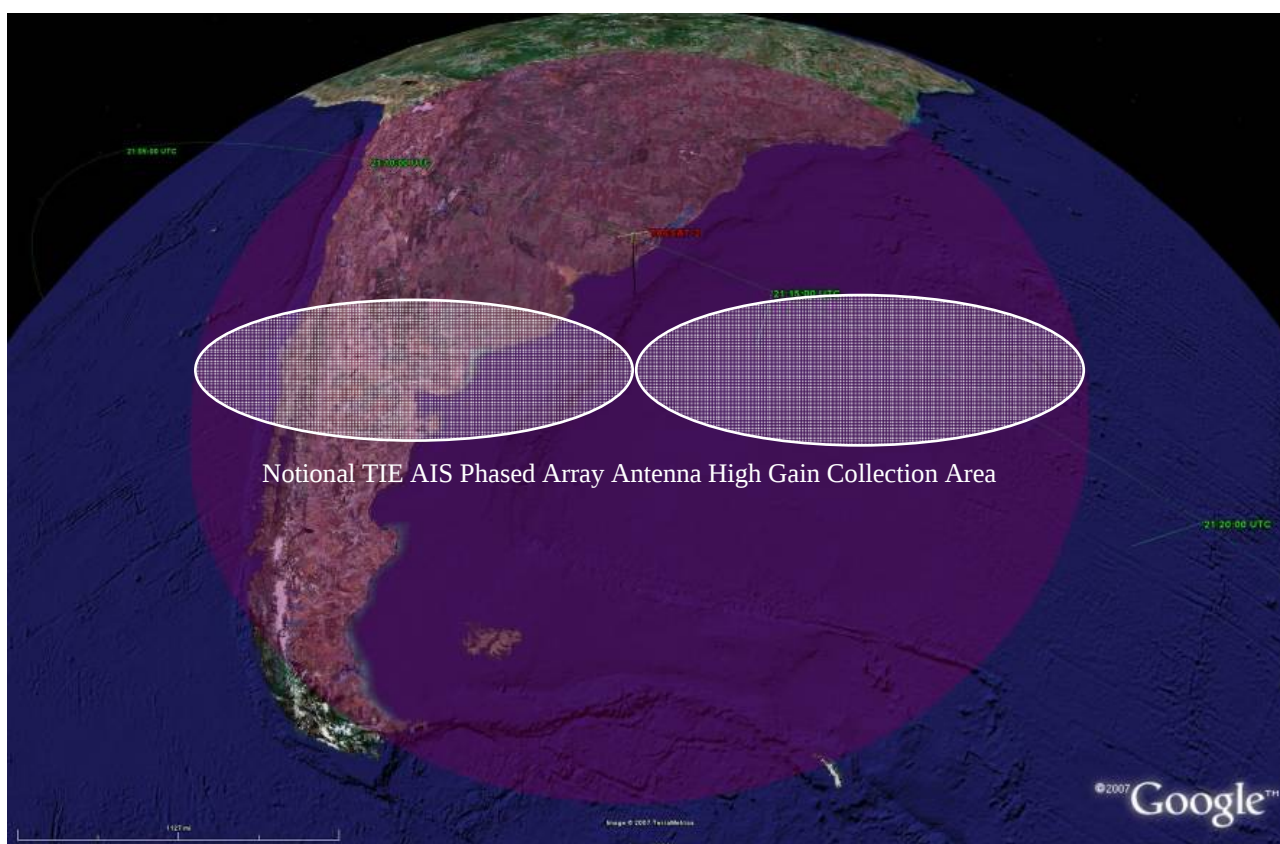
Figure 3. TIE AIS Phased Array Antenna Notional Instantaneous Field of View
