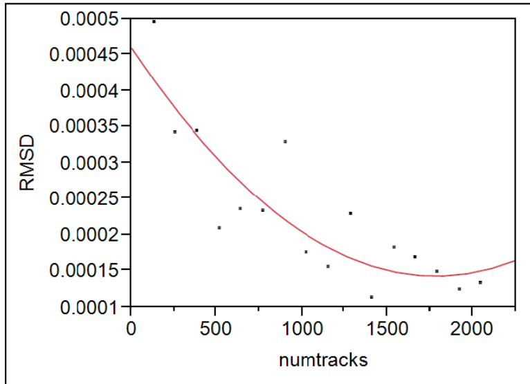
Figure 12. Effect of varying numtracks on RMSD for the 72-hour forecast probability field together with the best fit quadratic model. The model's R^2 is 0.757.
