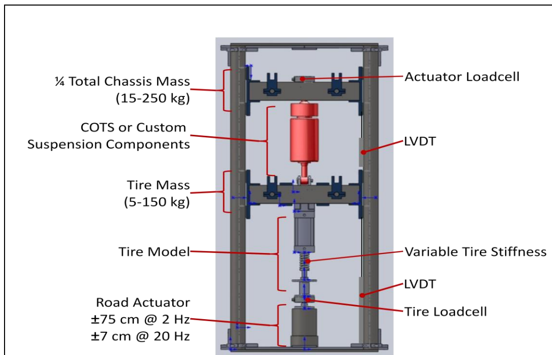
Figure 22. 2 DOF suspension test rig.
