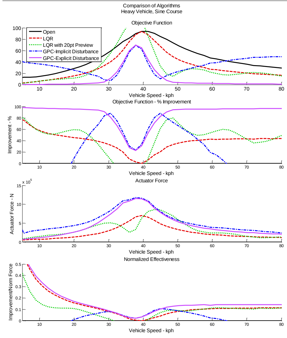
Figure 6. Comparison of control algorithms for Heavy Vehicle parameters on Sine course.
