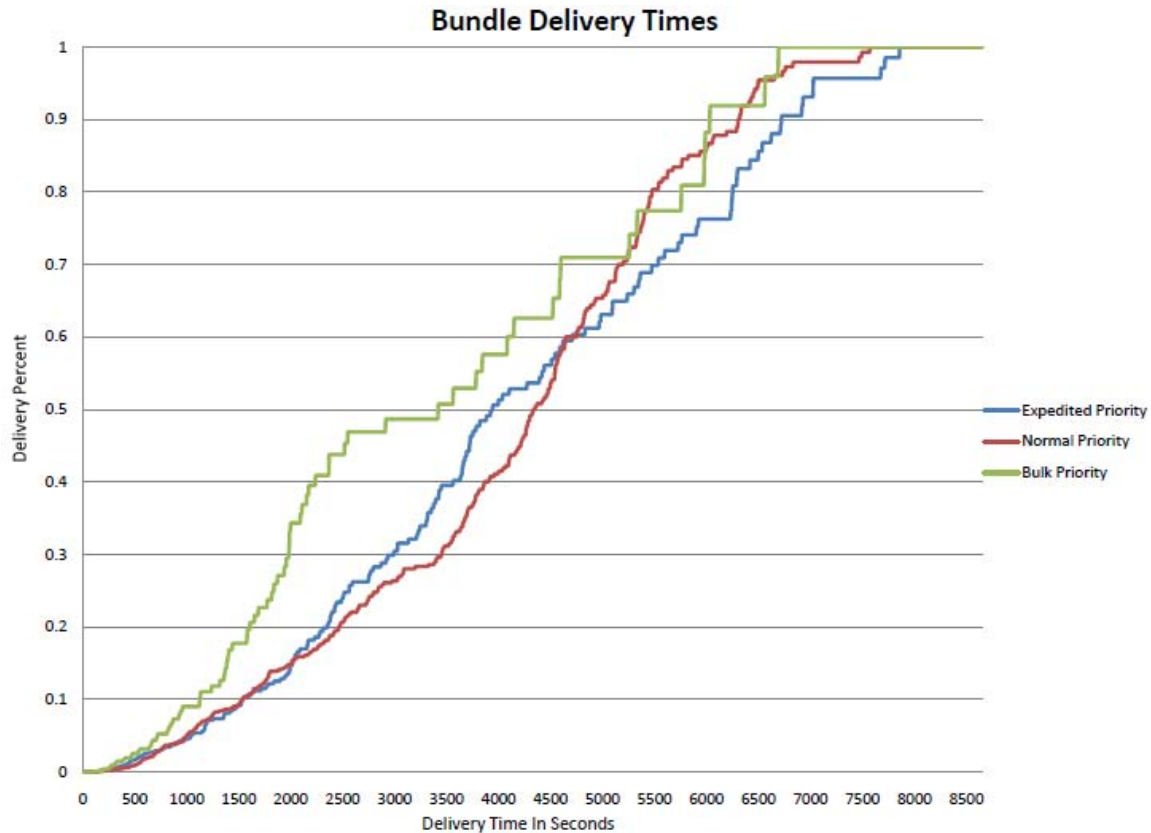
Figure 28: CDF of Delivery Times for the 10GB Queue Test Run Using COSFLEX and Priority
