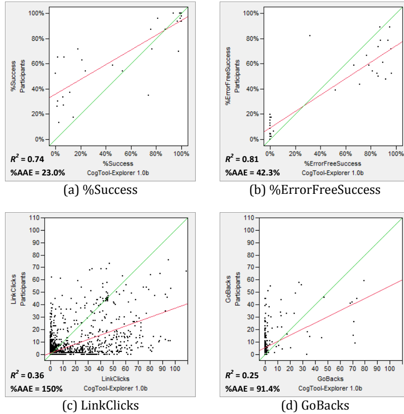
Figure 20: CogTool-Explorer 1.0b compared to participant data in the multi-page layout. Each data point in (a) and (b) represents a task, in (c) a link in a task, and in (d) a 2 nd -level page in a task. If model behavior perfectly matched participant data, all data points will lie on the green diagonal line. The red line is the best fitting line for the data points.
