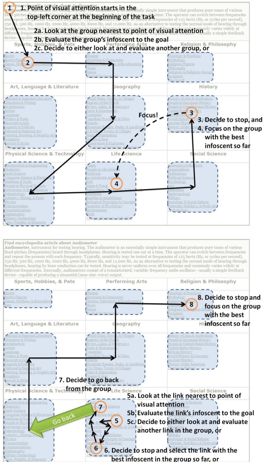
Figure 35: An example run of Consider Groups by CogTool-Explorer 1.2 in the multi-group layout.
