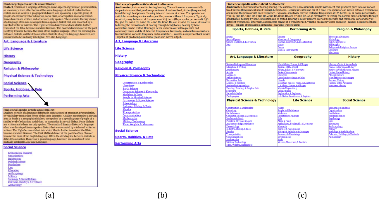
Figure 14: (a) The multi-page layout where each link in the top-level webpage (also referred to as a top-level link) led to its corresponding 2 nd -level webpage of links, (b) the half-flatten layout where selecting a top-level link reveals the 2 nd -level links grouped under that top-level link, and (c) the multi-group layout where the 2 nd -level links are grouped into nine groups.
