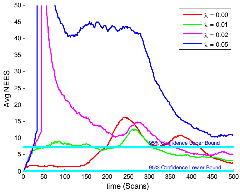
Figure 20. Average NEES for Algorithm II: 2D-4D LP, \sigma_q = 0.0005 .
