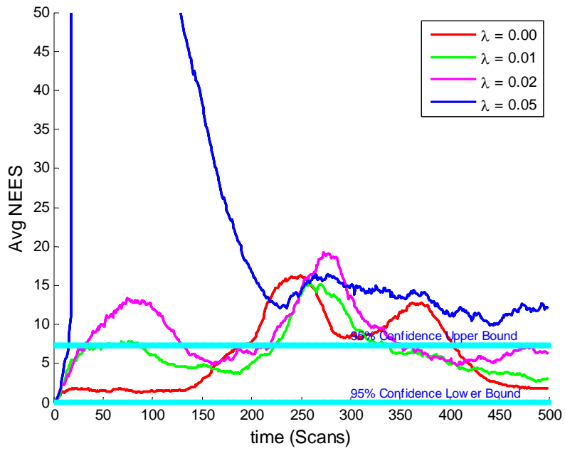
Figure 26. Average NEES for Algorithm II: 2D-3D LP, \sigma_q = 0.002 .
