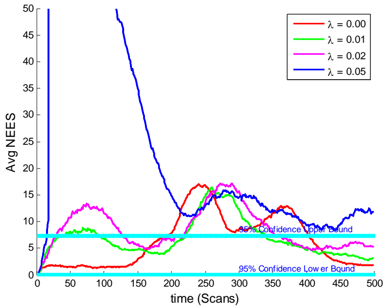
Figure 32. Average NEES for Algorithm II: 2D-11D LP, \sigma_q = 0.002 .
