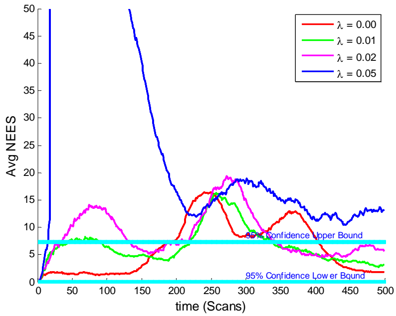
Figure 30. Average NEES for Algorithm II: 2D-6D LP, \sigma_q = 0.002 .
