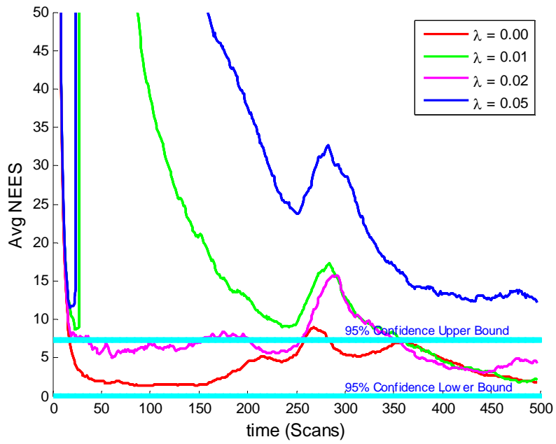
Figure 16. Average NEES for Algorithm I: 4D LP, \sigma_q = 0.0005 .
