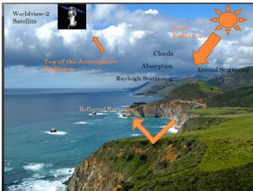
Figure 1. The solar irradiance transmission through the atmosphere.
