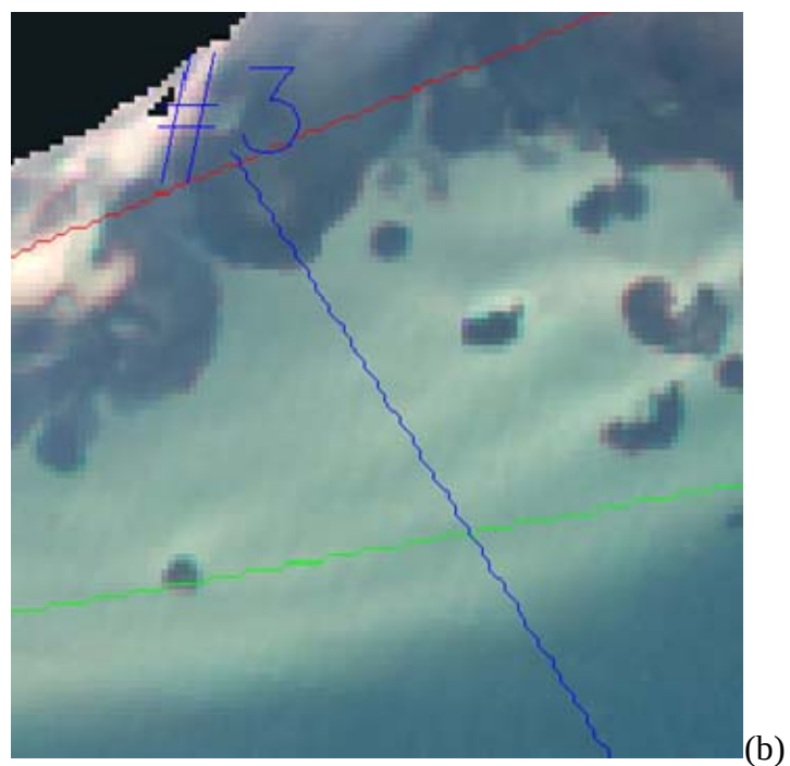
Figure 24. Magnification of Transect 3 (blue line) over the 116 m sand segment (pixels 18:67) where the shading indicates a wave-like pattern in the sand. The top (a) figure is a RGB reflectance composite and the bottom (b) figure is an YGB reflectance composite.
