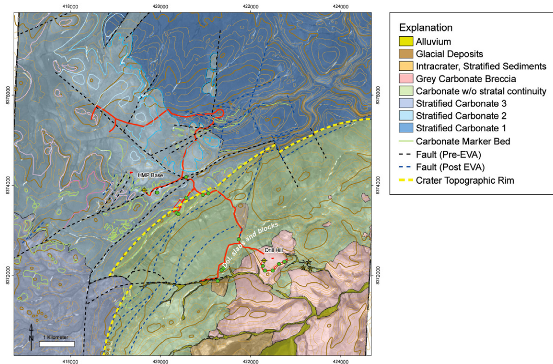
Figure 21. Revised geologic map. Green dots are sample localities. Blue dashed lines indicate new faults added to the original map. A glacial deposit is mapped and several distinct carbonate marker beds (pink, blue, and green lines beyond the crater rim) are now delineated.
