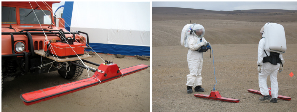
Figure 16. Ground-penetrating radar (GPR) at Houghton Crater. Left, a GPR is mounted on the front of a simulated pressurized crew rover; right, GPR is manually deployed by suited crew.
