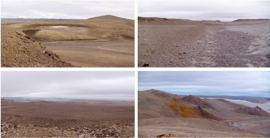
Figure 17. Four of the panoramas taken during the geologic mapping traverse. Top left: the rounded, brown, low relief terrain in the middle ground are the intra-crater stratified sediments; top-right: Contact between gray carbonate breccia (right) with unstratified intra-crater carbonate; bottom-left: view East into the crater from the rim near station 13; bottom-right: intra-crater gray carbonate breccia forms the distinctive white ridge in right middle of photo.
