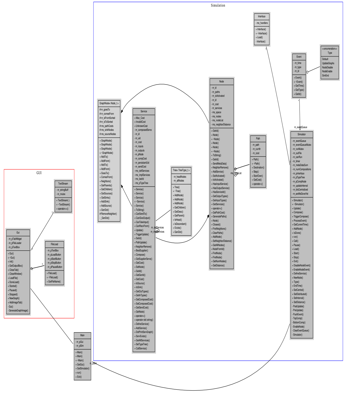
Figure 2.2 Class Diagram
