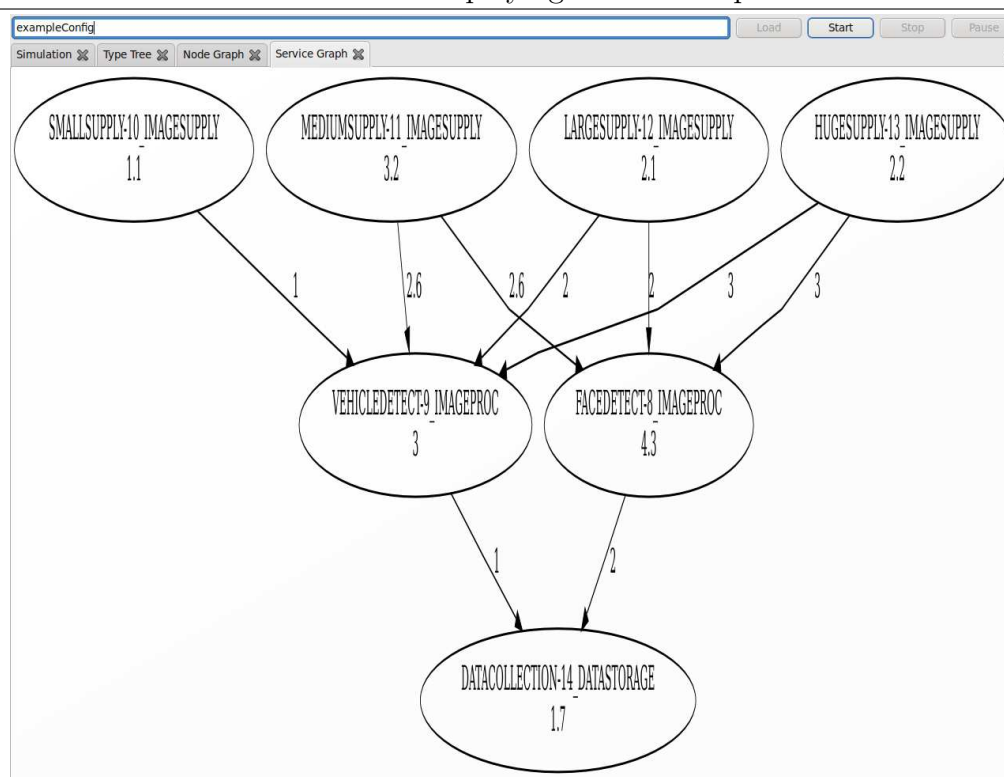
Figure 3.7 Simulator Screenshot: Displaying Service Graph
