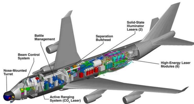
Figure 2. Airborne Laser Component Systems (Defense Industry Daily, 2009)
