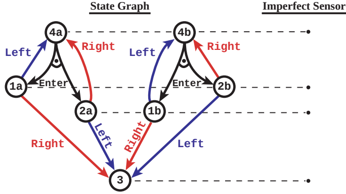
Figure 31: An imperfect sensor stratifies a graph into two subgraphs (the “a wing” and the “b wing”), over each of which sensing is effectively perfect.
