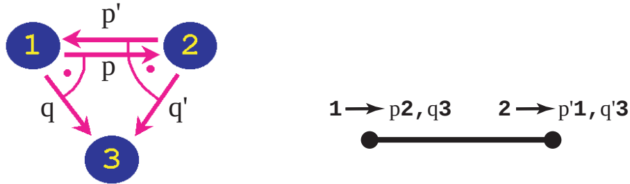
Figure 12: The graph on the left has two stochastic actions that together could create a cycle but must eventually converge to state 3. Consequently, the strategy complex on the right includes not only the individual actions but the full 1-simplex formed by these two actions.
