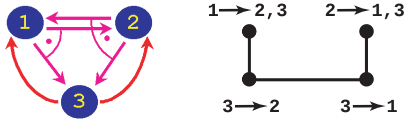
Figure 10: A loopback graph and loopback complex associated with the graph of Fig. 6. The complex is contractible.
