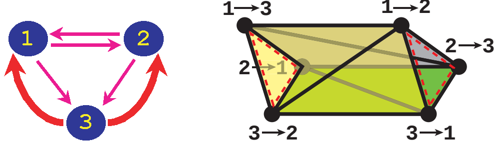
Figure 9: A loopback graph and loopback complex associated with the graph of Fig. 5. The complex contains 6 vertices, 12 edges, and 6 triangles (shaded). The two triangular endcaps outlined in dashed red are not part of the complex, since each gives rise to a cycle in the graph. The complex is homotopic to S^1 , the circle.
