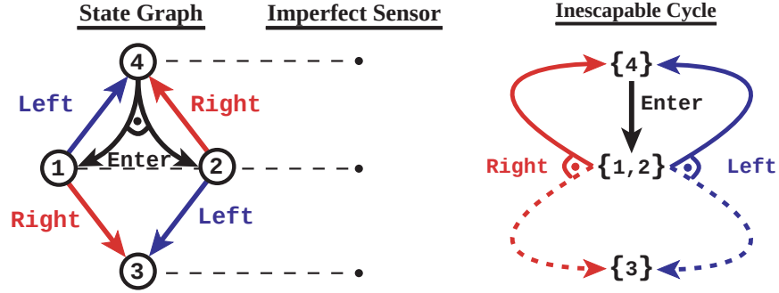
Figure 29: A graph, an imperfect sensor, and a potentially inescapable cycle between knowledge states \{4\} and \{1, 2\} (indicated by the solid arrows in the right panel).
