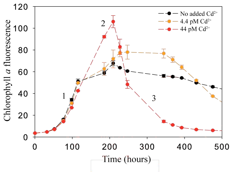
Figure 3.1: Growth of WH5701 under chronic Cd 2+ stress as measured by relative chlorophyll a fluorescence, points are averages of duplicates. This was a reconnaissance experiment in 28 mL tubes. Error bars represent range of duplicate measurements. Note 1) similar growth rate through exponential phase 2) increased maximum chlorophyll a fluorescence with added Cd 2+ and 3) increased mortality rates with added Cd 2+ . These are physiological effects.
