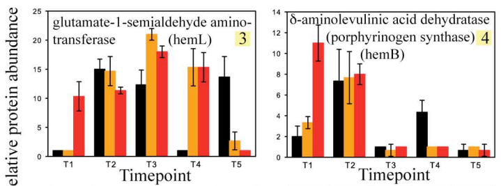
Figure 3.8: Relative protein abundances of chlorophyll biosynthesis proteins. Pathway from Blankenship 2002. Error bars represent standard deviation of triplicate injections.
