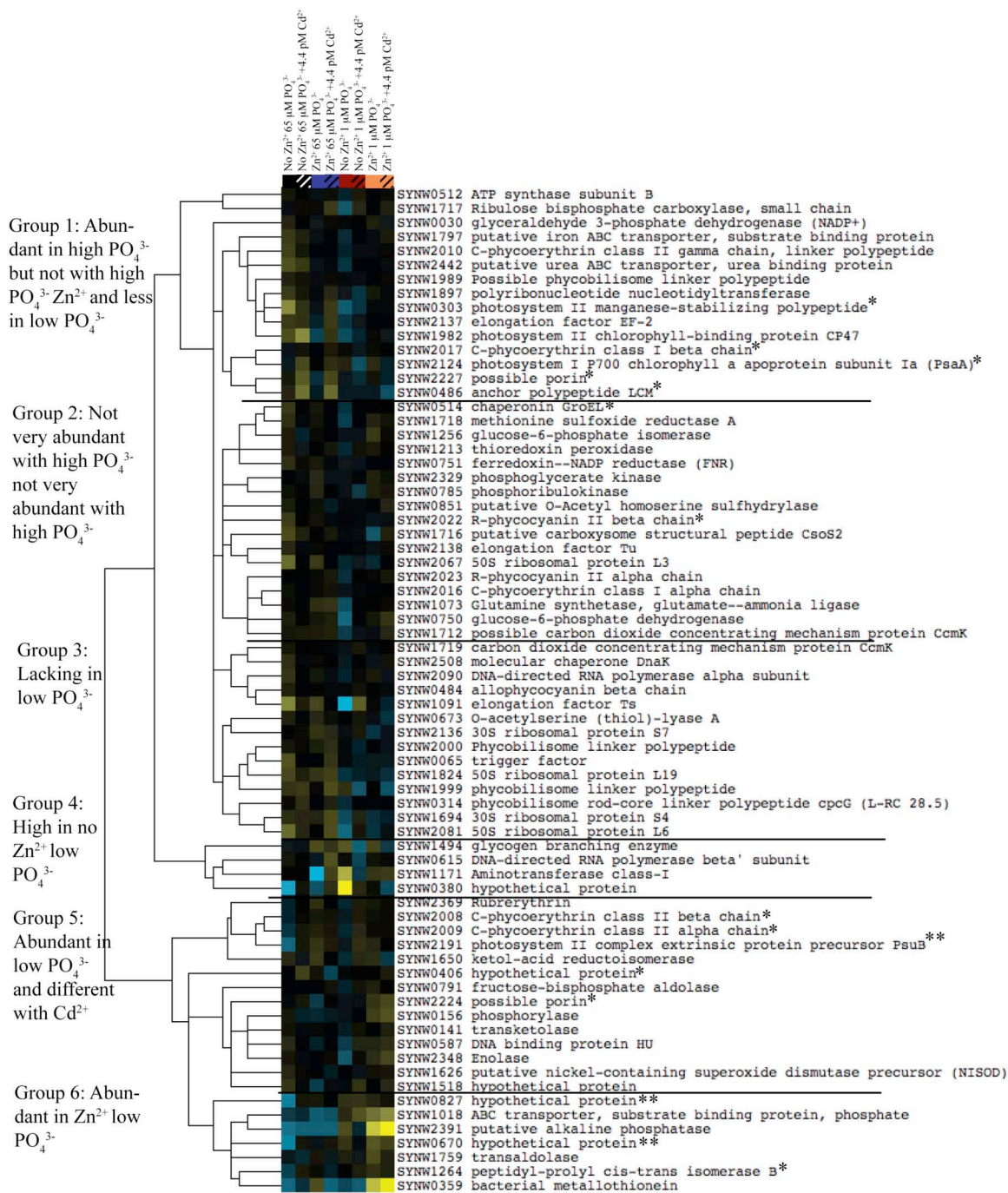
Figure 4.7: Cluster analysis of relative protein abundance. No Zn^{2+} 65 \mu M PO_4^{3-} , Zn^{2+} 65 \mu M PO_4^{3-} , No Zn^{2+} 1 \mu M PO_4^{3-} , Zn^{2+} 1 \mu M PO_4^{3-} and these four chronic treatments with 4.4 pM Cd^{2+} acutely added. Four low, 1 \mu M PO_4^{3-} on the right and replete, 65 \mu M PO_4^{3-} on the left. There are 71 proteins. Proteins are averages of duplicates have at least 7 counts and are different by a value of 7. Data are log transformed, centered, clustered by Kendall's Tau, centroid linkage. Yellow = more abundant, Blue = less abundant, * = statistically different by Fisher's Exact Test between the No Zn^{2+} 65 \mu M PO_4^{3-} and the No Zn^{2+} 65 \mu M PO_4^{3-} + 4.4 pM Cd^{2+} ** = differentially abundant by two-fold or greater and statistically different by Fisher's Exact Test between the No Zn^{2+} 65 \mu M PO_4^{3-} and the No Zn^{2+} 65 \mu M PO_4^{3-} + 4.4 pM Cd^{2+} .
