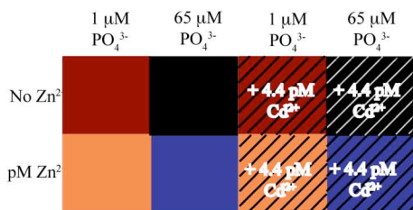
Figure 4.10: Relative protein abundance of proteins \geq two-fold greater in abundance and/or statistically different by Fisher's Exact Test in the no \text{Zn}^{2+} added 65 \mu\text{M} \text{PO}_4^{3-} + 4.4 pM \text{Cd}^{2+} compared to the no \text{Zn}^{2+} added 65 \mu\text{M} \text{PO}_4^{3-} treatments. Error bars are the standard deviation of duplicate injections.
