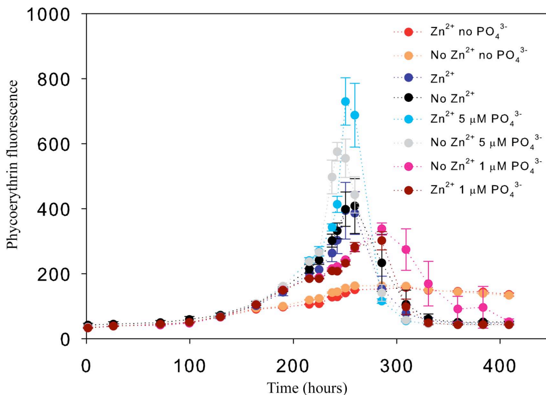
Figure III.1: Phycoerythrin fluorescence vs. time, chronic PO 4 3- limitation reconnaissance study. Error bars are one standard deviation of triplicate 28 mL tubes. Note that no PO 4 3- added treatments, both with and without Zn 2+ appear to have a stationary phase. 1 μM PO 4 3- treatments appear to have a brief stationary phase and then enter death phase, the Zn 2+ dying faster than the no added Zn 2+ . The 5 μM PO 4 3- treatments fluoresced to a greater maximum than the 65 μM PO 4 3- . This phenomenon is thus far unexplained and was not observed in a concurrent 500 mL experiment (four treatments, 1 and 65 μM PO 4 3- with and without Zn 2+ ).
