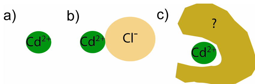
Figure 1.2: Cd^{2+} in the dissolved phase in seawater. a) Cd^{2+} as a free ion. b) Cd^{2+} complexed with Cl^- to form CdCl^+ (and other chlorocomplexes) c) Cd^{2+} bound to organic ligands of uncertain structure and origin. Inorganic Cd^{2+} is mostly present as CdCl^+ in seawater, although Cd^{2+} has been found to be 70% bound to organic ligands in some surface waters. Cd^{2+} and CdCl^+ are considered to be labile and bioavailable. Cd bound to organic ligands is not thought to be bioavailable.
