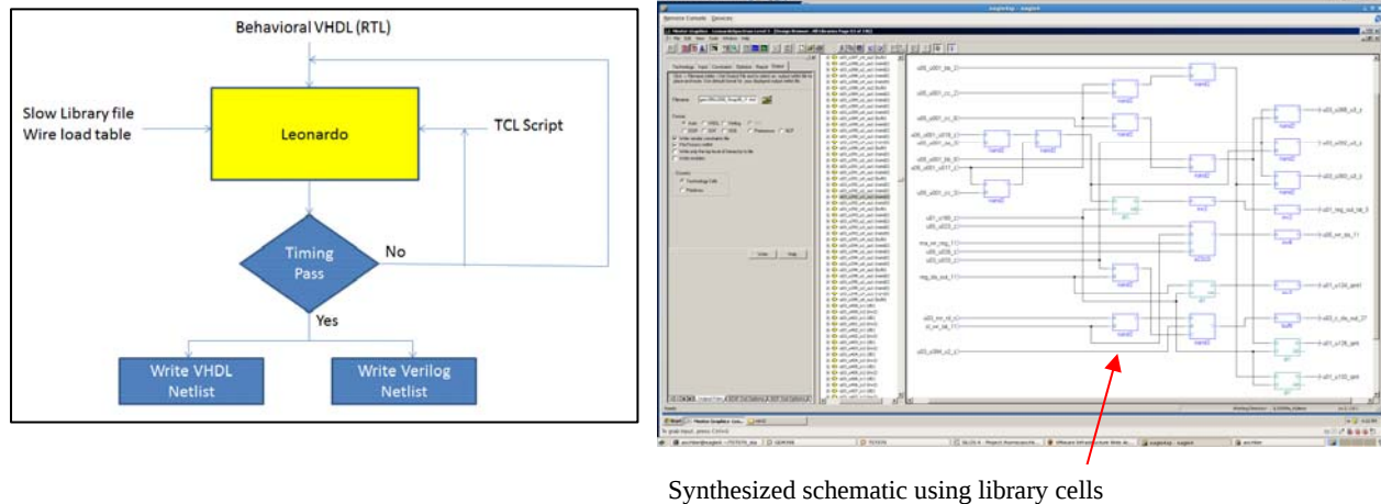
Figure 2.8 – Synthesis Flow (Leonardo)
