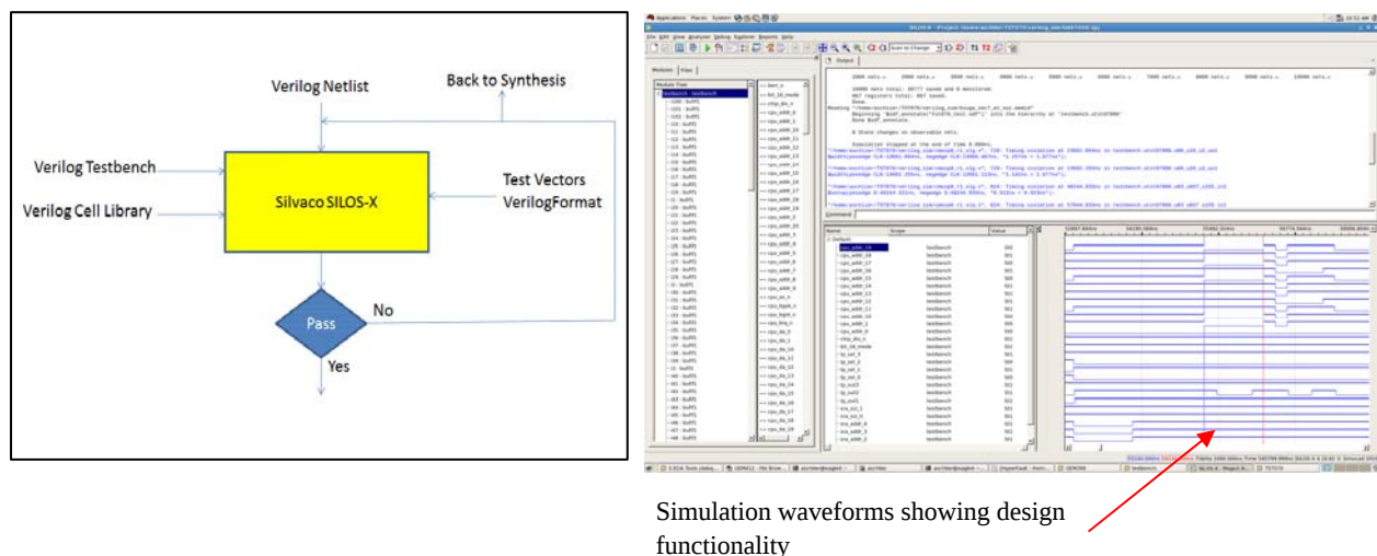
Figure 2.9 – Synthesized netlist validation using Silos-X
