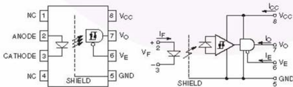
Figure 17. Schematic diagram of optocoupler (From: [12]).
