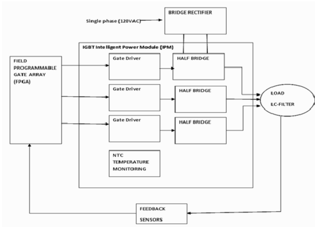
Figure 3. VSI IPM module diagram.
