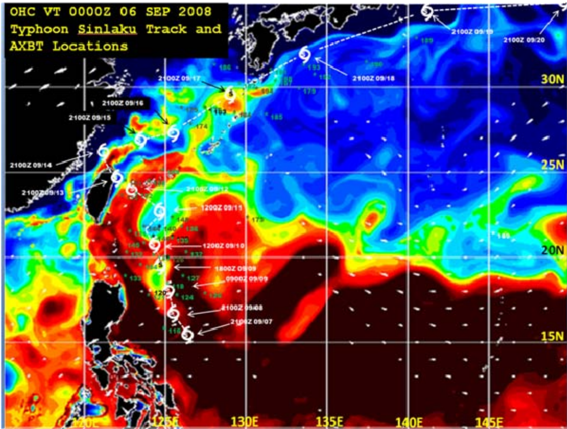
Figure 17. Ocean Heat Content ( \text{kJ cm}^{-2} ) at 0000 UTC 6 September 2008 superimposed with TY Sinlaku storm track and AXBT locations.
