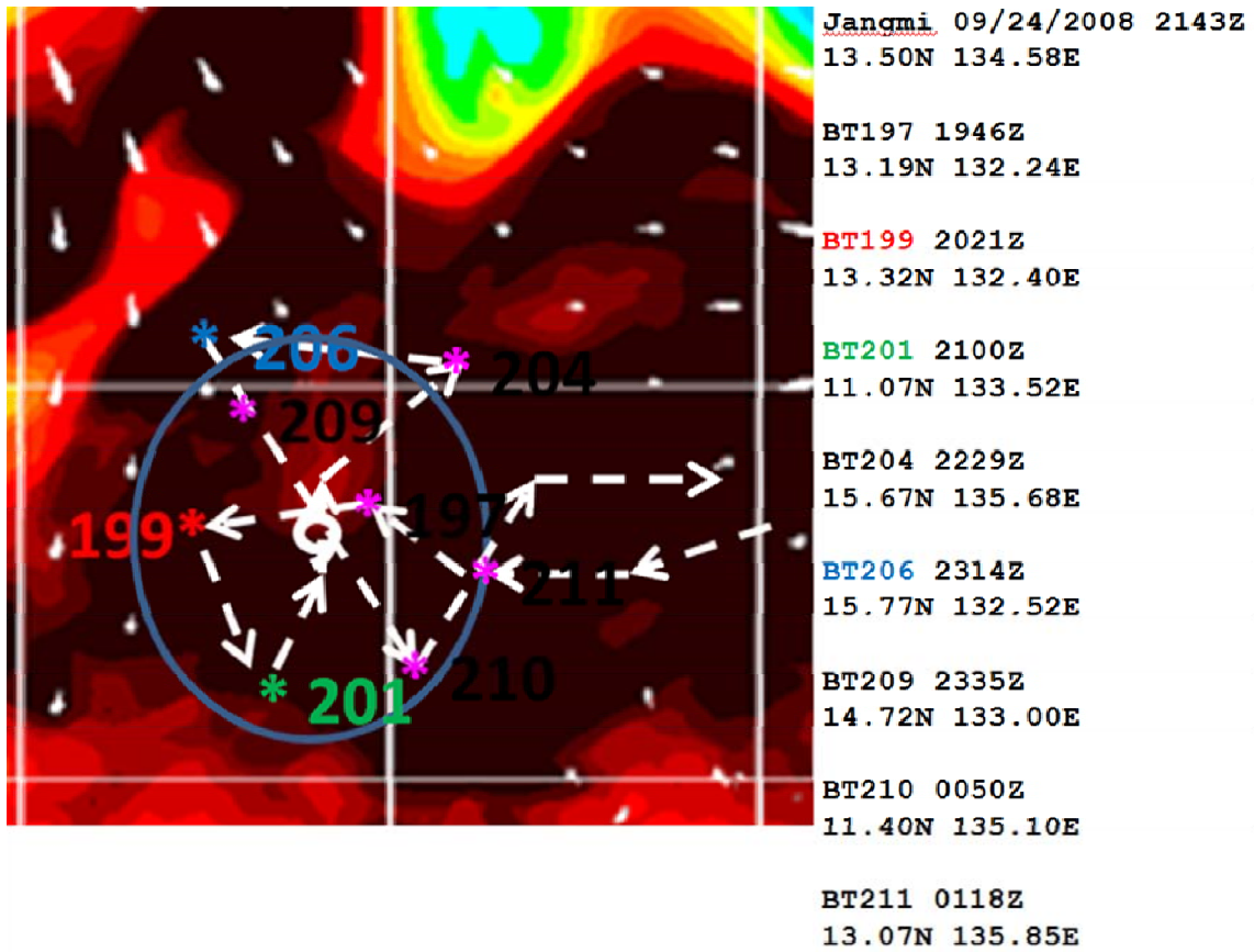
Figure 49. Composite plot of AXBTs in relation to TY Jangmi at 2143 UTC 24 September 2008 and overlaid on the EASNFS OHC analysis at 0000 UTC 23 September 2008. Arrows correspond to the aircraft flight track.
