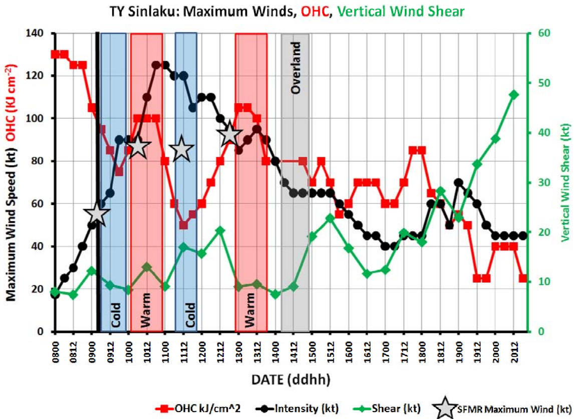
Figure 28. Typhoon Sinlaku OHC (kJ cm -2 ) values from EASNFS analysis, intensities (kt) in 6-h increments, vertical wind shear (kt) in 12-h increments from ECMWF analysis, and SFMR maximum winds (kt). Colored boxes define periods when Sinlaku traversed significant ocean features or land.
