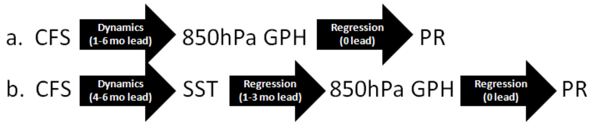
Figure 30. Two potential variations of the S-D approach to producing LRFs of Jul-Aug Pakistan PR. (a) At leads of 1–6 months, use a dynamical model (e.g., CFS) to predict 850 hPa GPH in Jul-Aug, then use the predicted GPH to force a regression model that predict Jul-Aug Pakistan PR. (b) At leads of 4–6 months, use a dynamical model (e.g., CFS) to predict SST at leads of 1–3 months, then use the predicted SST as the predictor in a regression of 850 hPa GPH in Jul-Aug, and then use the predicted GPH in a regression to predict Jul-Aug Pakistan PR.
