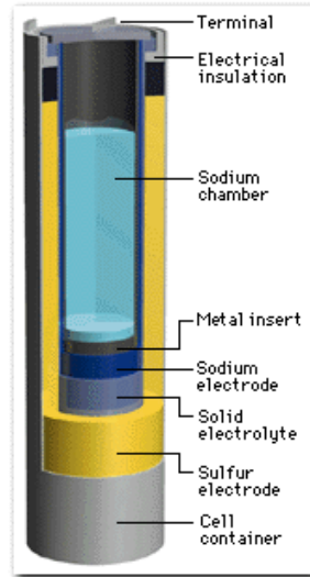
Figure 11. Sodium sulfur battery. (From [34])
