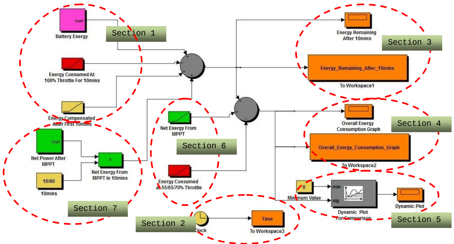
Figure 55. Simulation model with solar panel.
