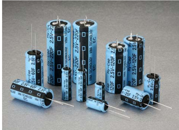
Figure 17. Super-capacitors. (From [50])
