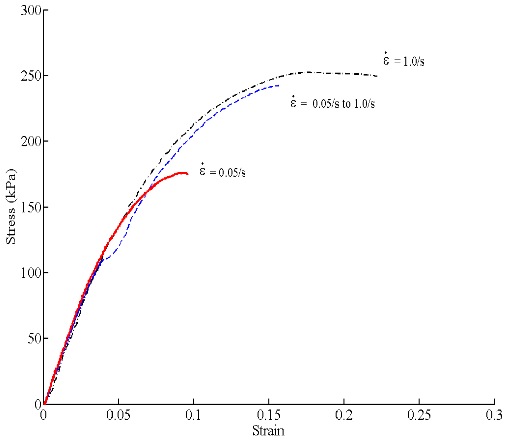
Figure 28. Typical stress-strain curve under two strain rates.
