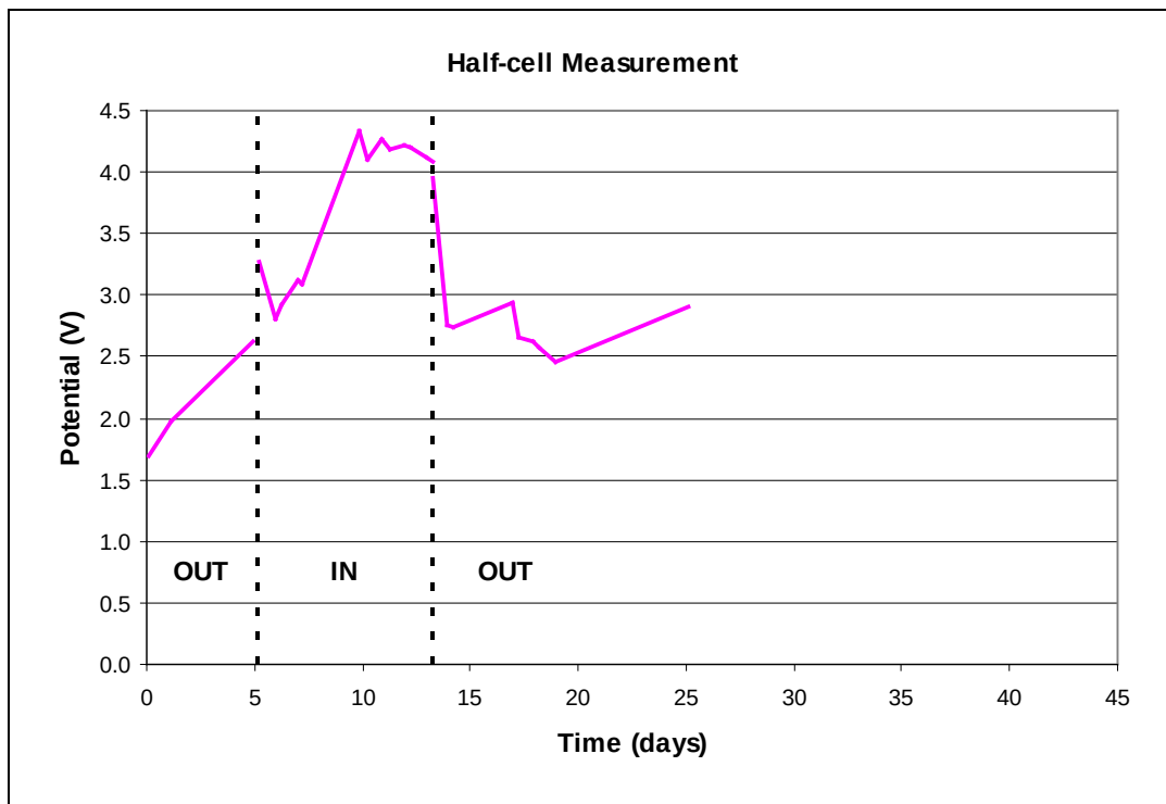
Figure C-18. Half-cell steel (rebar) corrosion and gas generation potential measurements when cathodes are placed inside (IN) and outside (OUT) ring ground.
