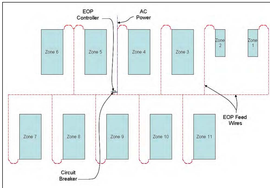
Figure E-21. EOP zone layout.
