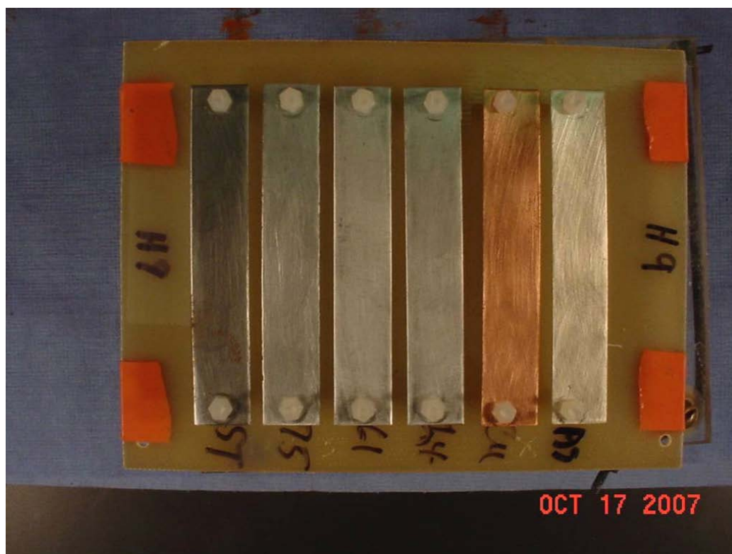
Figure 3.5. Test samples after 3 months inside ECM, June – August 2007.
