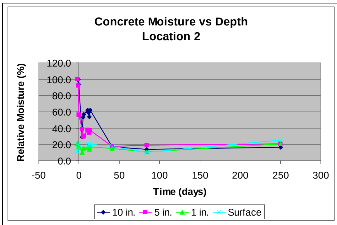
Figure E-52. Plot of concrete moisture over time at location 2, Figure E-43.
