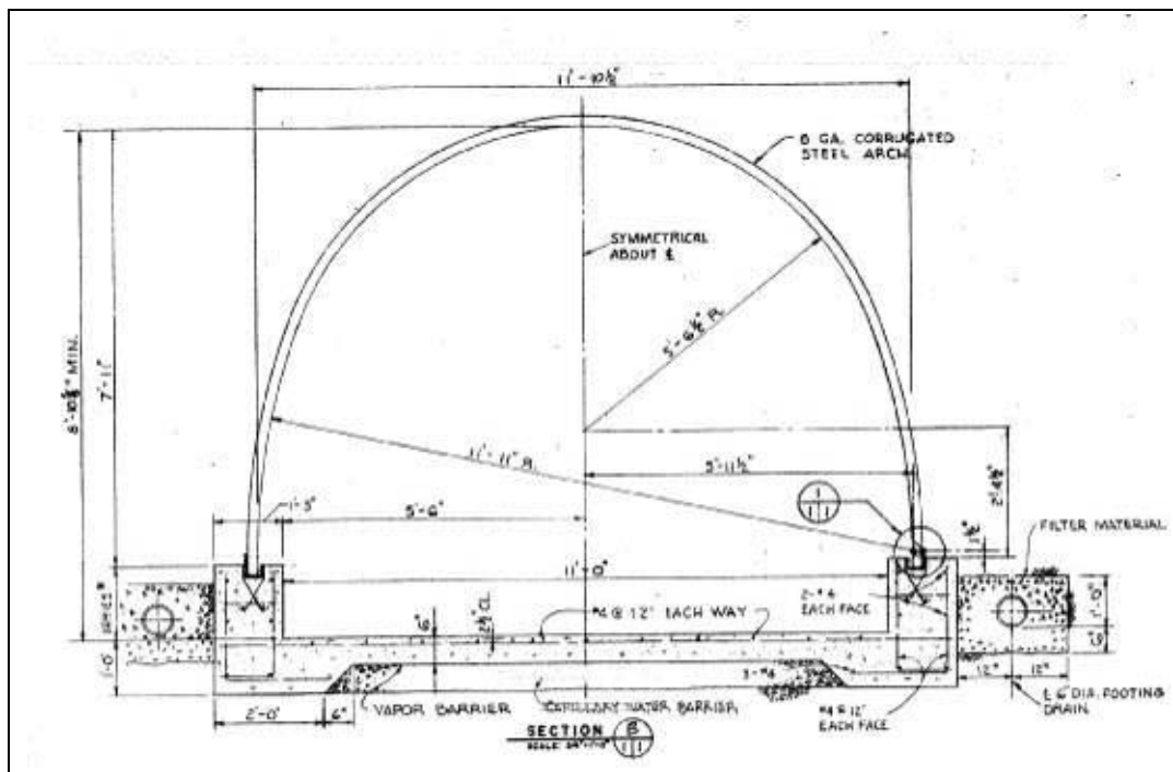
Figure E-30. Standard drawing for a steel arch ECM.
