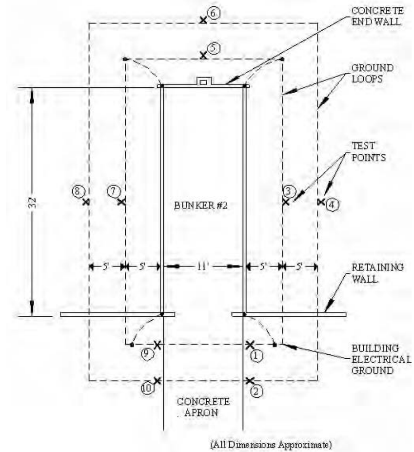
Figure E-43. Location of ground test points on bunker 2.
