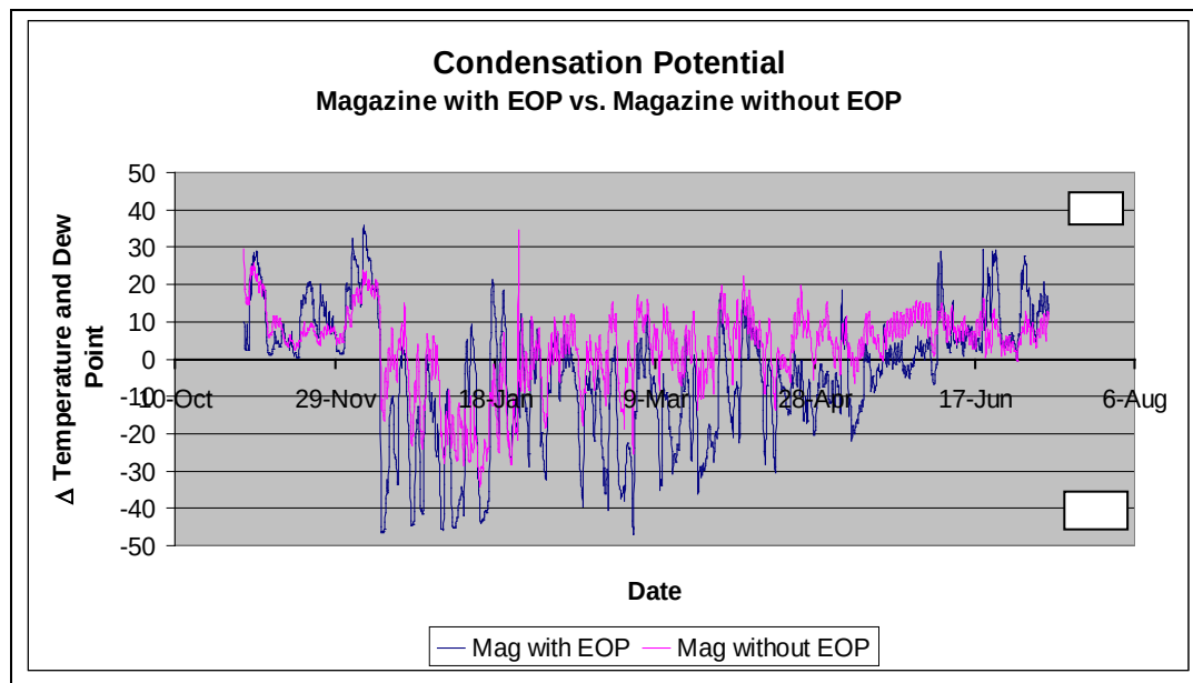
Figure E-57. Plot of condensation potential temperature for magazine with and without EOP vs time.
