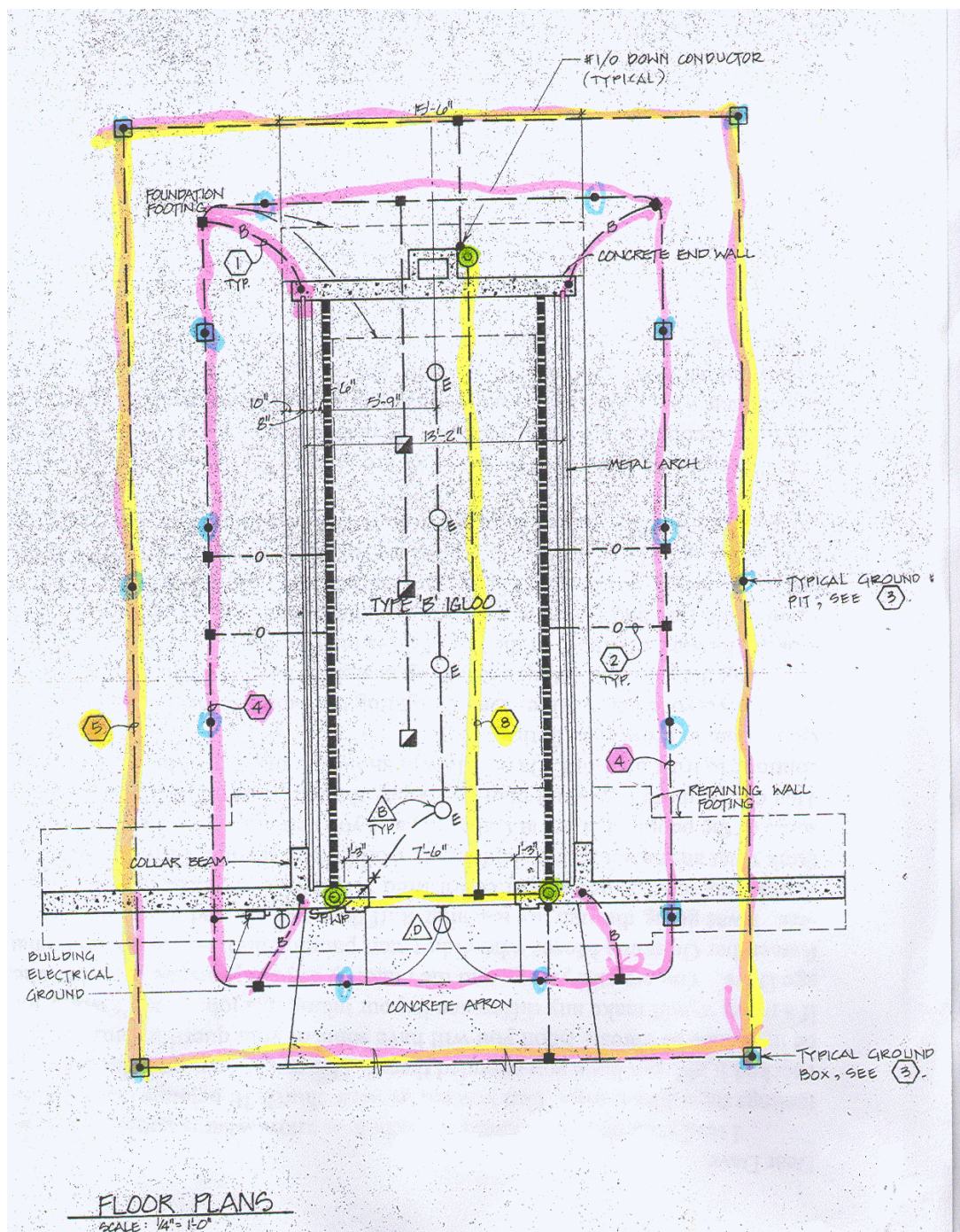
Figure C-1. Type 'B' Igloo Floor Plans. The pink highlighted ground loop approximates that installed in the model.
