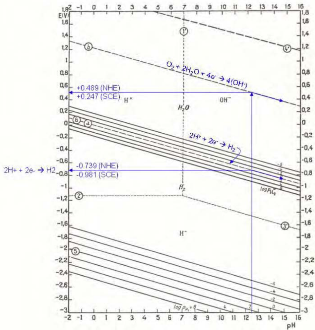
Figure E-34. potential-pH equilibrium diagram for the system hydrogen-water, at 25 °C.
