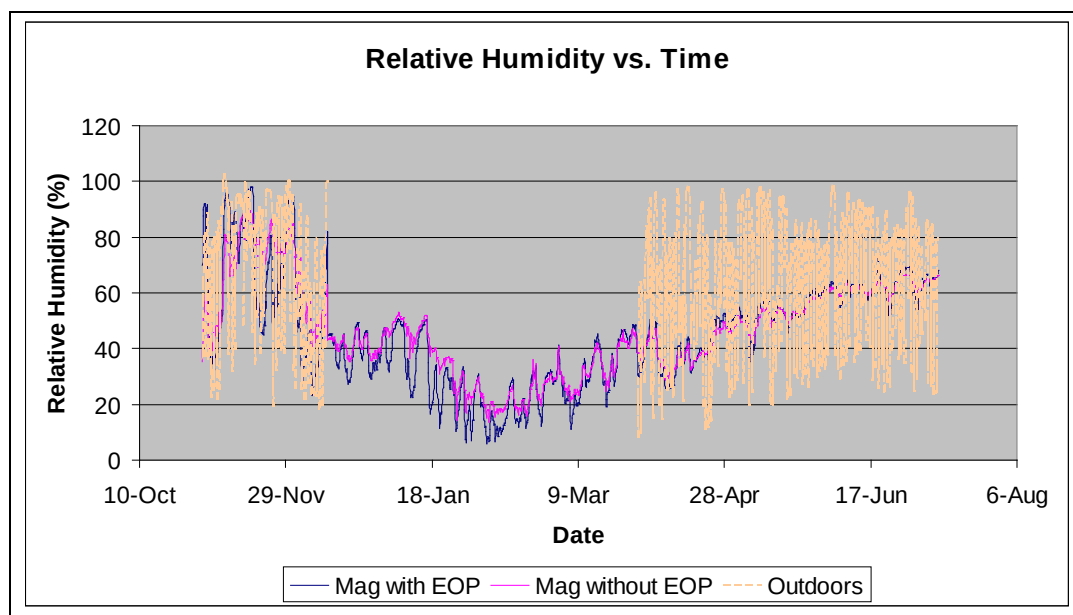
Figure E-56. Plot comparing outdoor relative humidity with interior relative humidity for magazine with and without EOP vs time.
