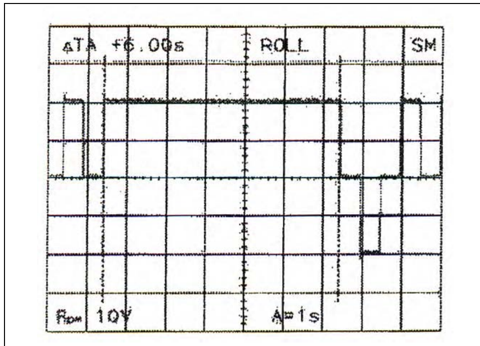
Figure E-25. Plot of EOP pulse (voltage along vertical axis and time along horizontal axis).
