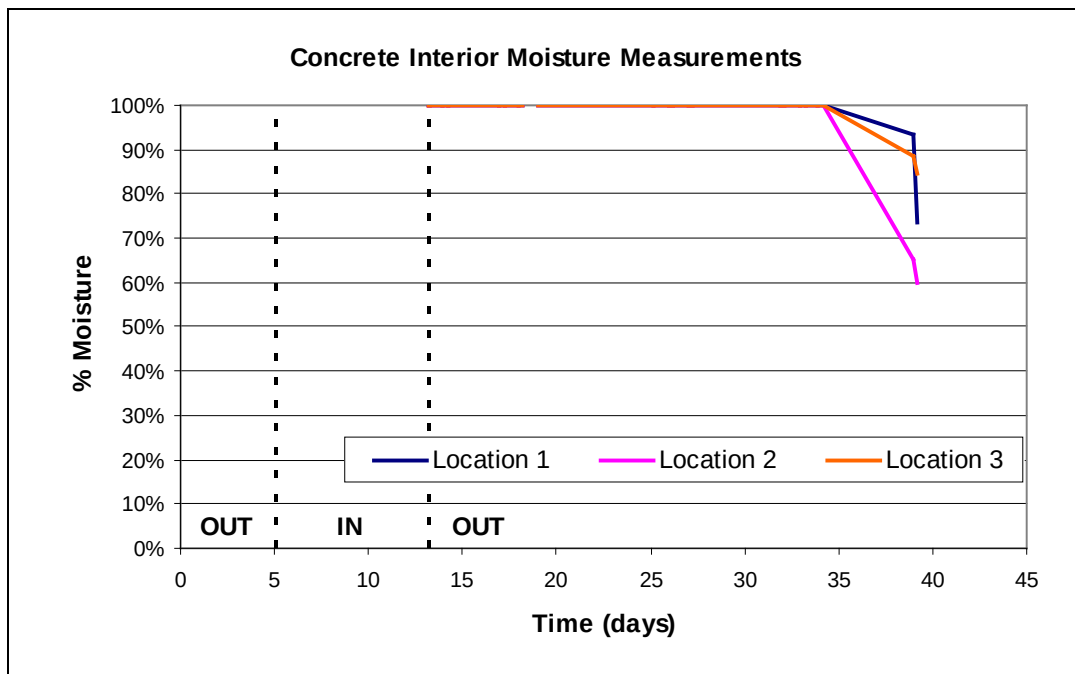
Figure C-20. Concrete interior moisture (Protimeter) when cathodes are placed outside (OUT) of ring ground.
