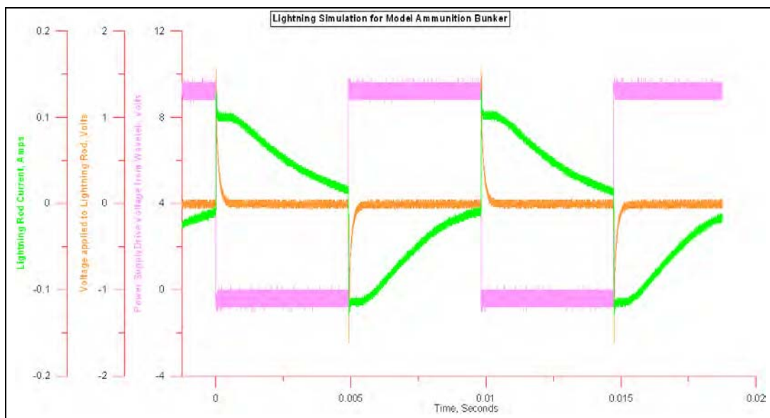
Figure C-11. Source signal for simulated lighting measurements on ECM model.
