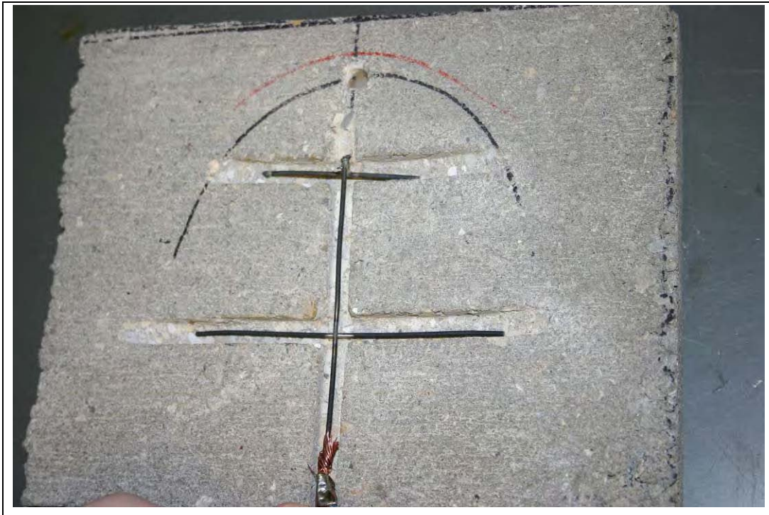
Figure C-4. Rear wall section with anodes in grooves.
