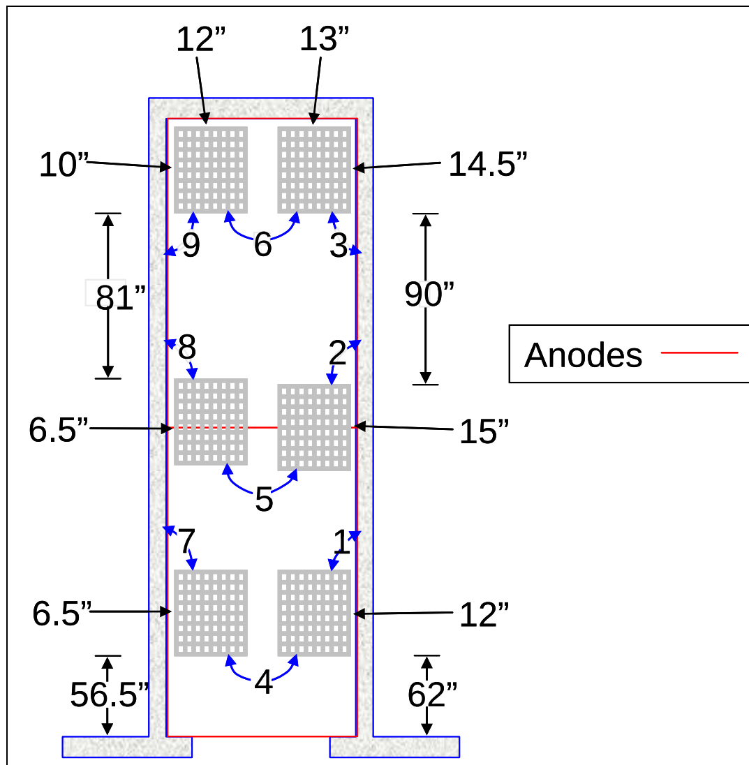
Figure E-32. Drawing indicating locations of metal pallets in magazine and electrical potential measurement locations.
