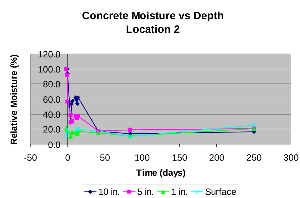
Figure 3.3. Plot of concrete moisture over time at location 2 (Figure E-42).
