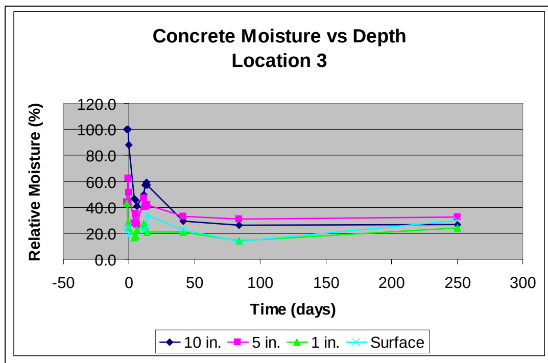
Figure E-53. Plot of concrete moisture over time at location 3, Figure E-43.
