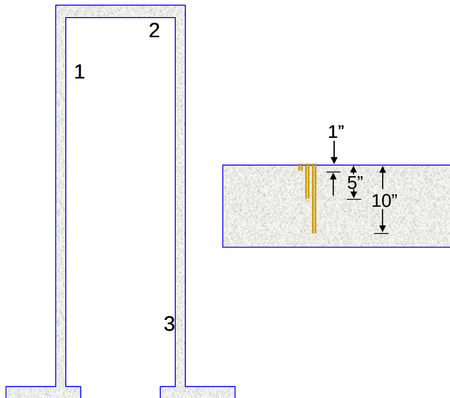
Figure E-42. Diagram of concrete moisture test locations and measurement setup.
