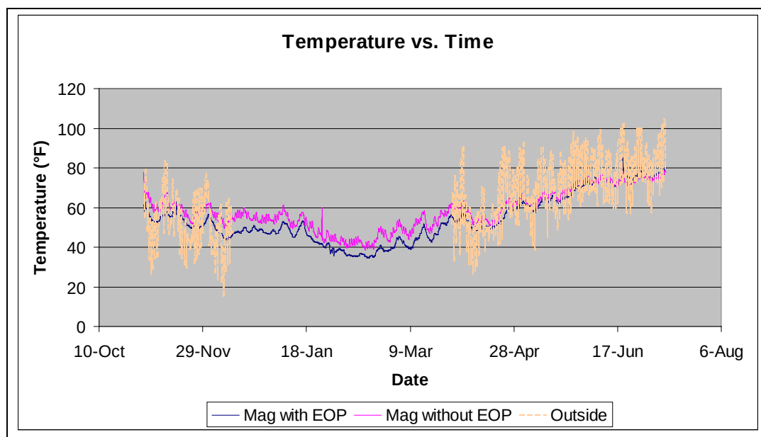
Figure E-54. Plot comparing outdoor temperature with interior temperature for magazine with and without EOP vs time.
