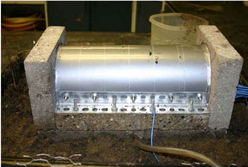
Figure 3.1. Laboratory model of ECM used for initial safety testing.
