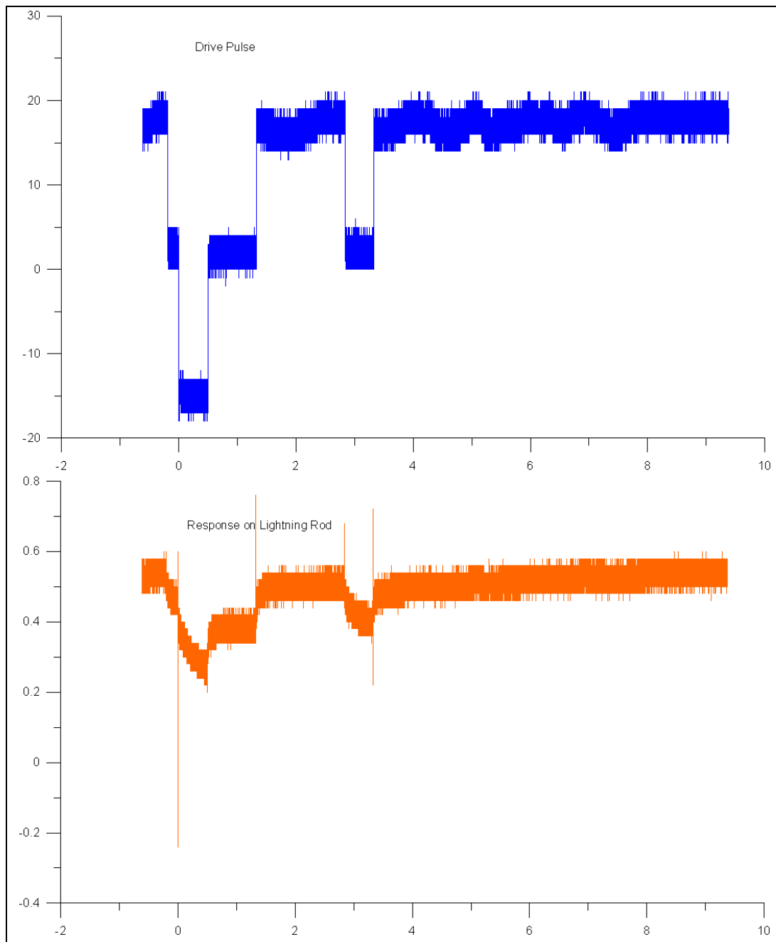
Figure C-12. EOP circuit current coupling to grounding system.
