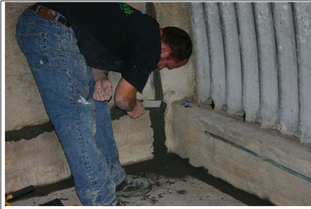
Figure E-11. Anode being grouted in slot.
