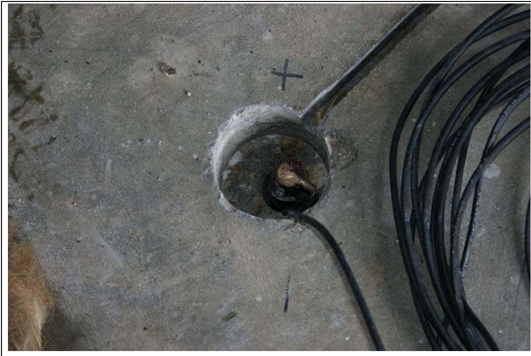
Figure E-13. Cathode lead wire exothermic weld connection.
