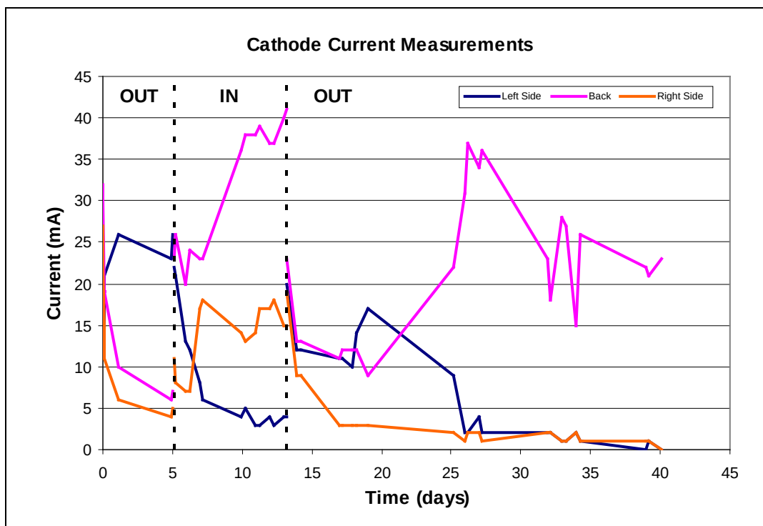
Figure C-16. Cathode currents when cathodes are placed inside (IN) and outside (OUT) ring ground.
