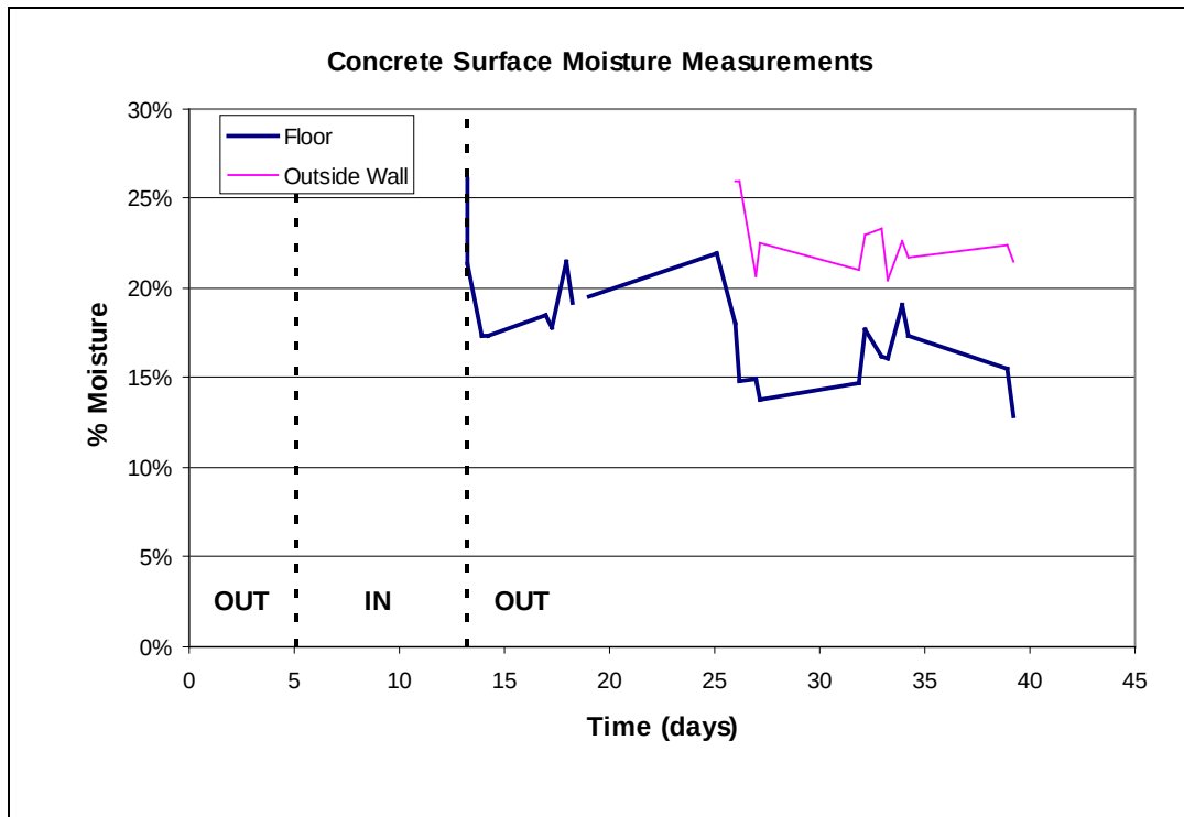
Figure C-19. Surface moisture (Protimeter) when cathodes are placed outside (OUT) of ring ground.
