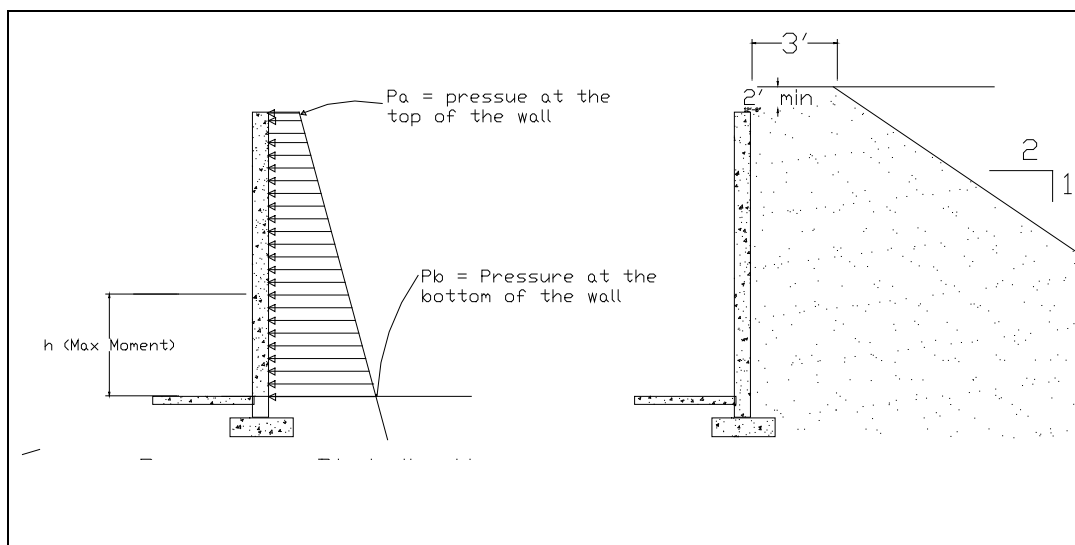
Figure D-2. Pressure distribution of the soil on the back wall of the igloo.
