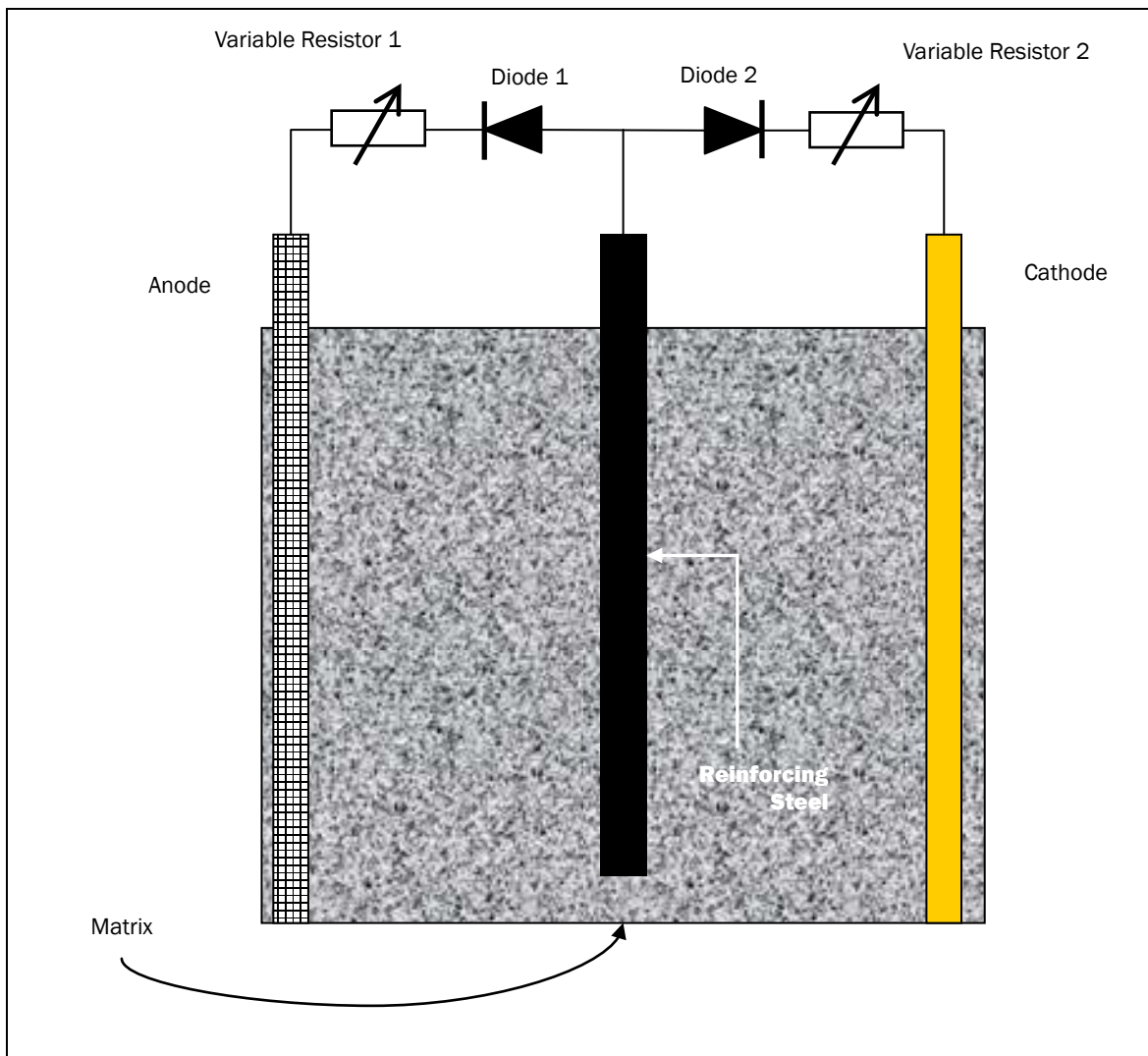
Figure E-38. Diagram illustrating stray current corrosion protection circuitry.
