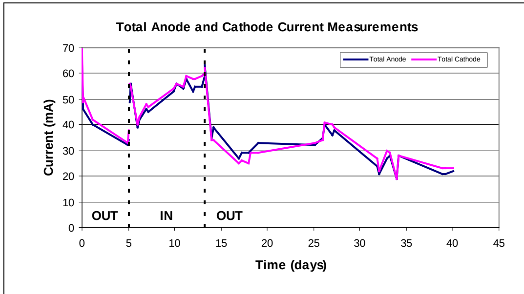
Figure C-17 Total anode and cathode current when cathodes are placed inside (IN) and outside (OUT) ring ground.
