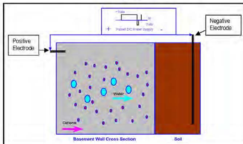
Figure 1-1. Electro-Osmotic Pulse Waveform and Movement of Water through Concrete.
