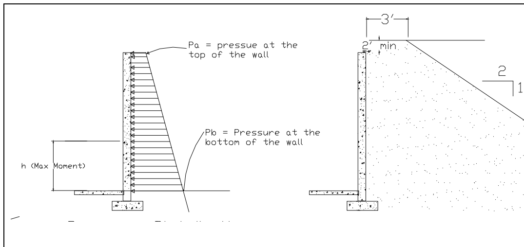
Figure D-5: Pressure Distribution of the Soil on the Back Wall of the Igloo.
