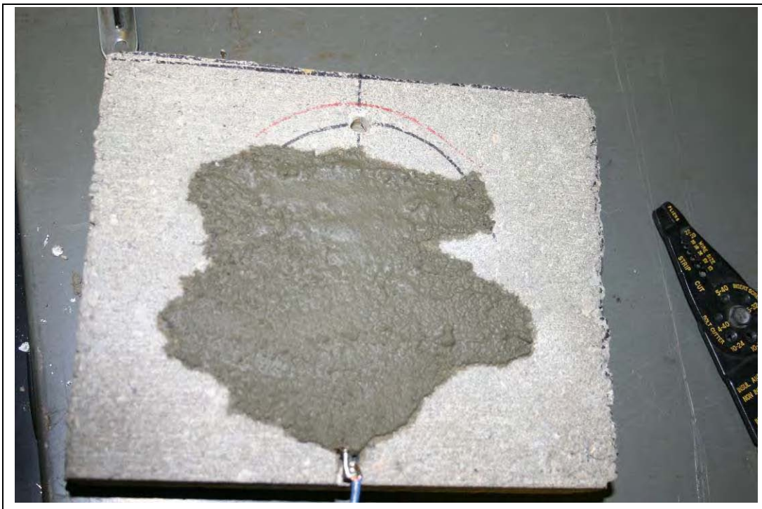
Figure C-5. Rear wall with grouted anode.
