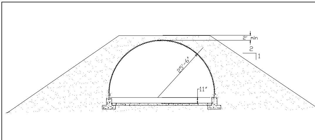
Figure D-4: Section in a typical ammunition and explosive storage magazine.
