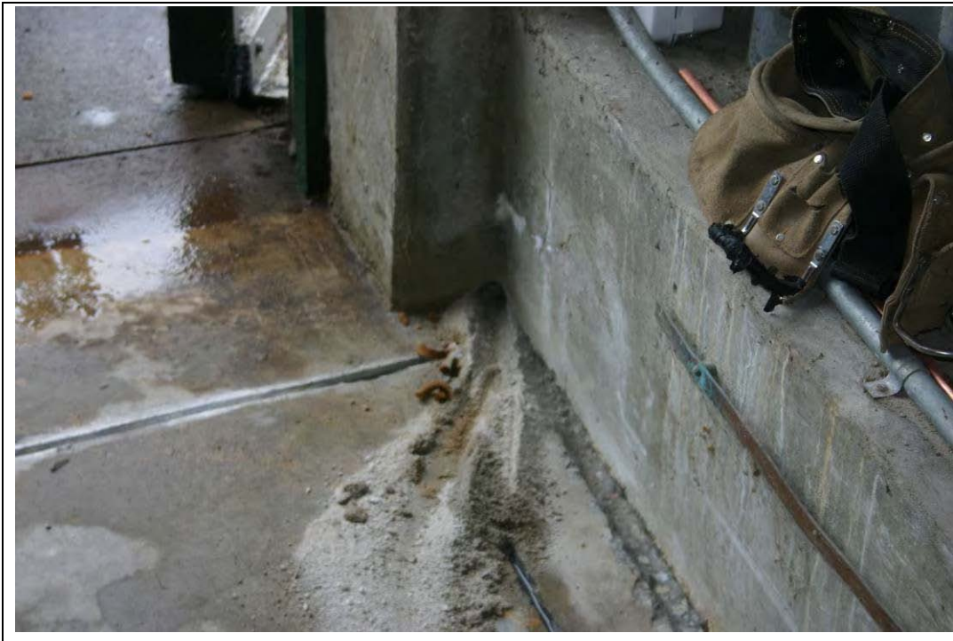
Figure E-17. Hole through head wall for lead wires.
