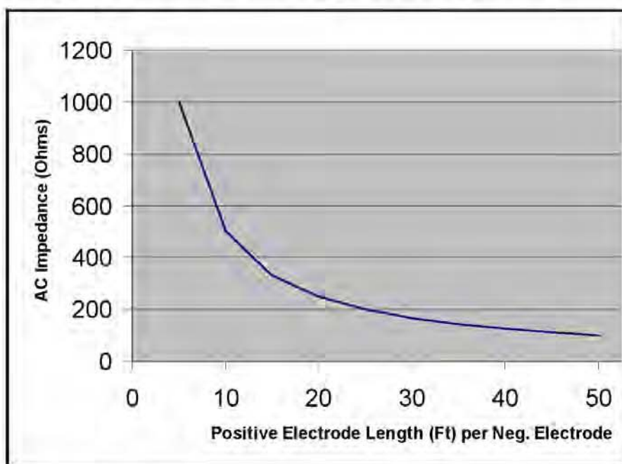
Figure 2-1. Maximum Positive to Negative Electrode Resistance.
