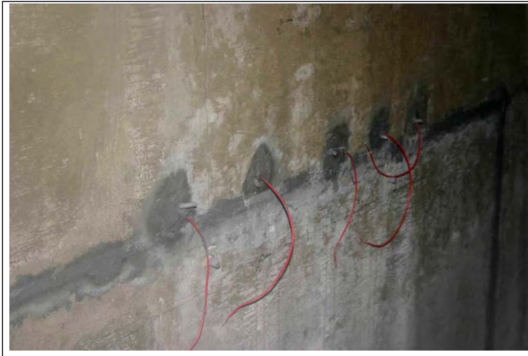
Figure E-41. Photograph of stray-current test setup.
