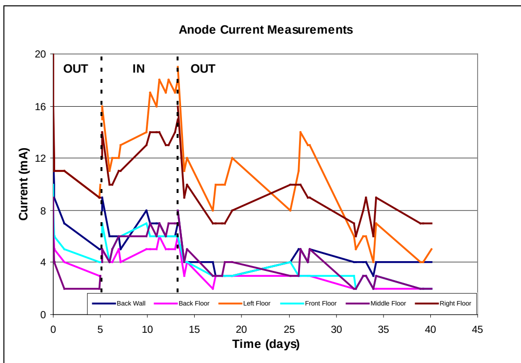
Figure C-15. Anode currents when cathodes are placed inside (IN) and outside (OUT) ring ground.
