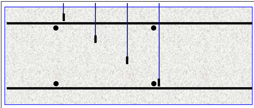
Figure E-40. Diagram of stray-current test setup.
