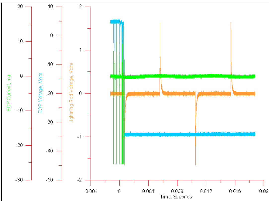
Figure C-13. "Lightning rod" induced grounding system current coupling to EOP circuit.
