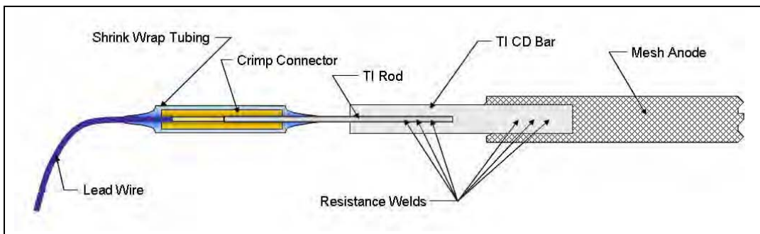
Figure E-10. Sketch of anode lead wire connection.
