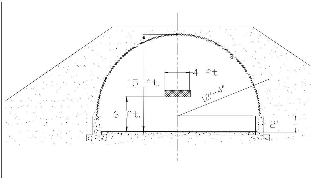
Figure D-3. Area of maximum moment on the back wall.
