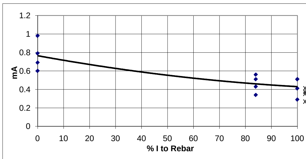
Figure E-50. Corrosion current on rebar probe when connected to EOP system negative as a function of current flow.
