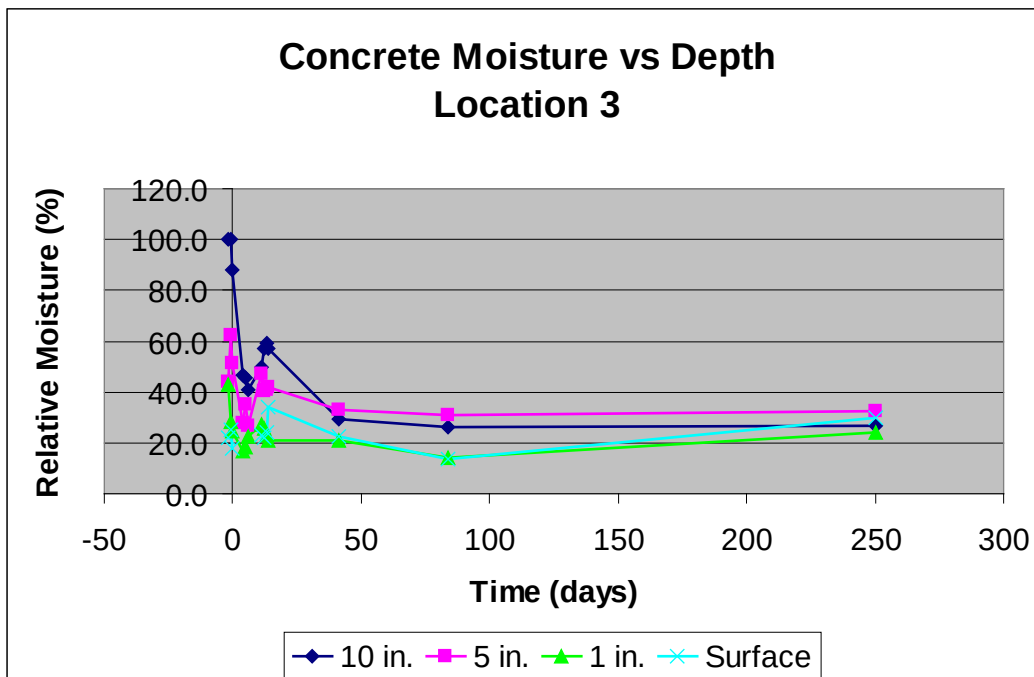
Figure 3.4. Plot of concrete moisture over time at location 3 (Figure E-42).
