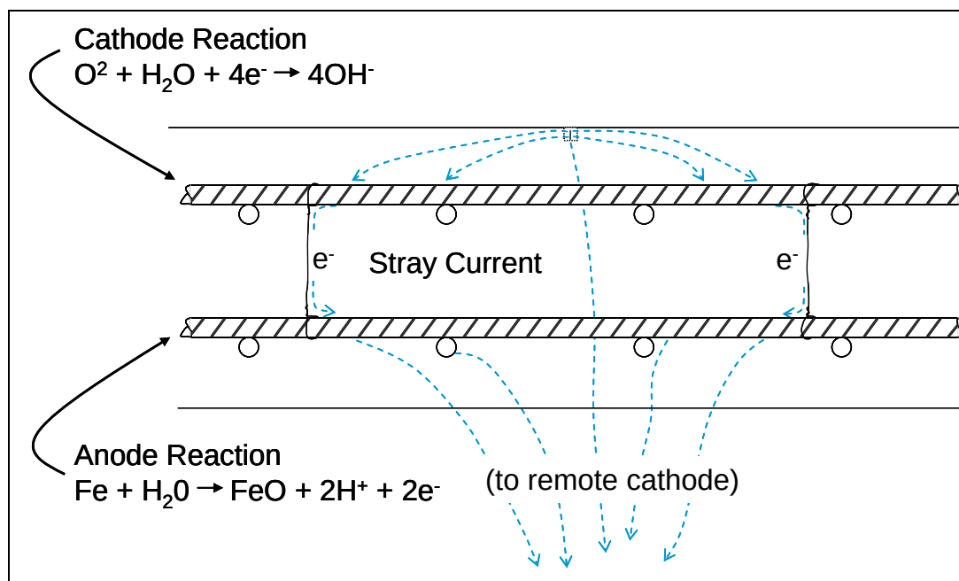
Figure E-37. Diagram of stray current corrosion mechanism.
