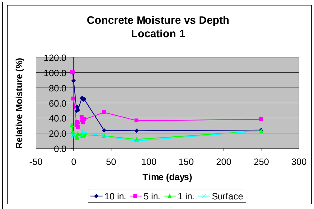
Figure E-51. Plot of concrete moisture over time at location 1, Figure E-43.
