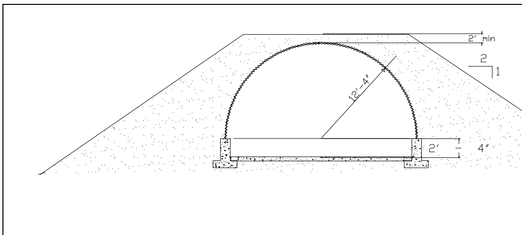
Figure D-1. Section in a typical ammunition and explosive storage magazine.
