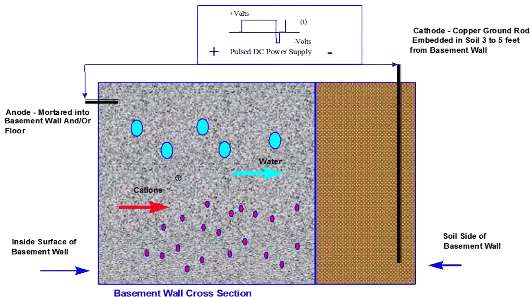
Figure 2: Schematic diagram of the Electro-Osmotic Pulse system.
