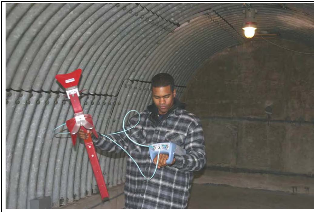
Figure E-47. Test apparatus to detect and measure radio frequency output.
