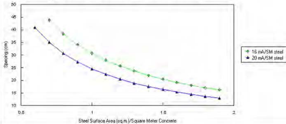
Spacing for ELGARD 150 Ribbon Mesh
