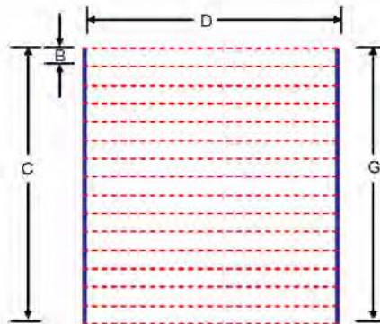
Free Body Diagram: Feed Anodes from Both Ends
