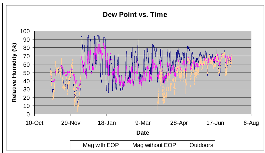
Figure E-55. Plot comparing outdoor dew point with interior dew point for magazine with and without EOP vs time.
