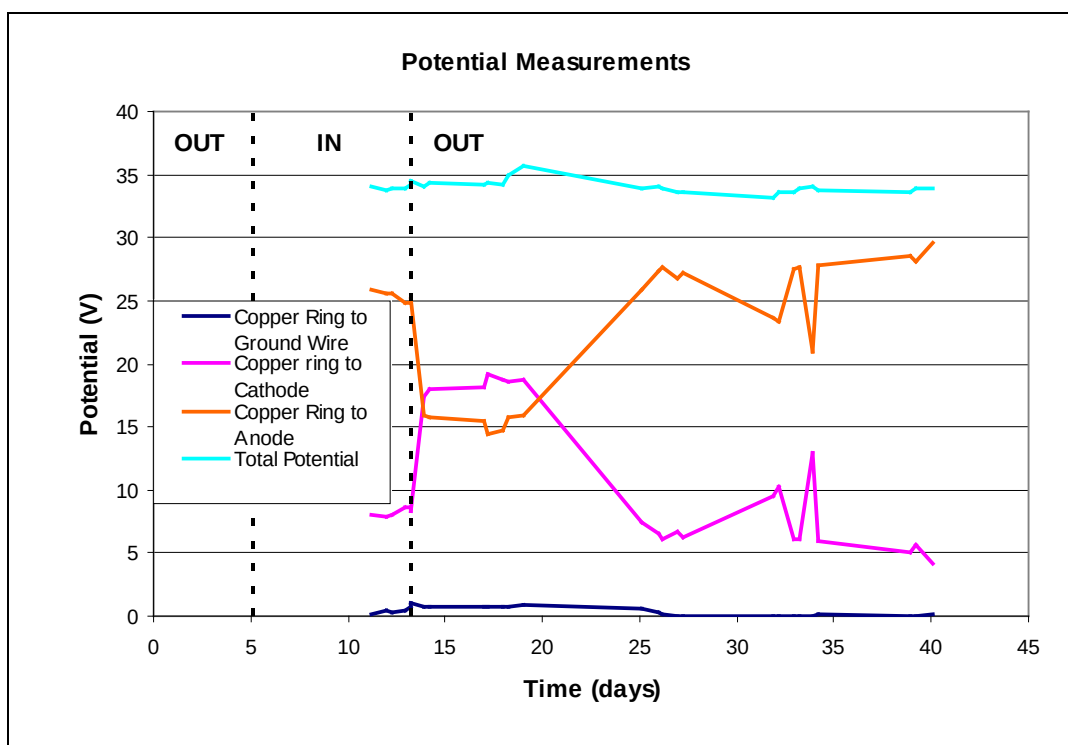
Figure C-14. Electrical potentials between conductors when cathodes are inside (IN) and outside (OUT) ring ground.
