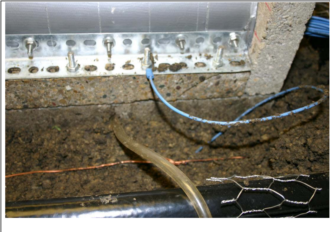
Figure C-8. ECM model with bare copper wire ground exposed.
