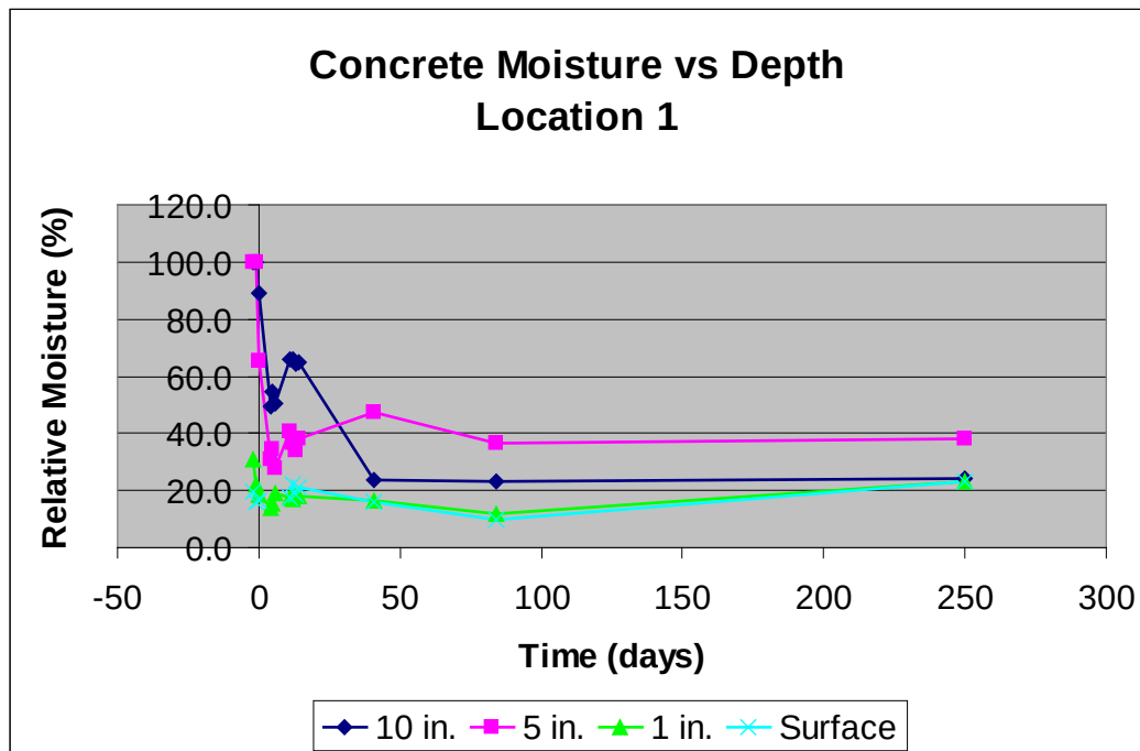
Figure 3.2. Plot of concrete moisture over time at location 1 (Figure E-42).
