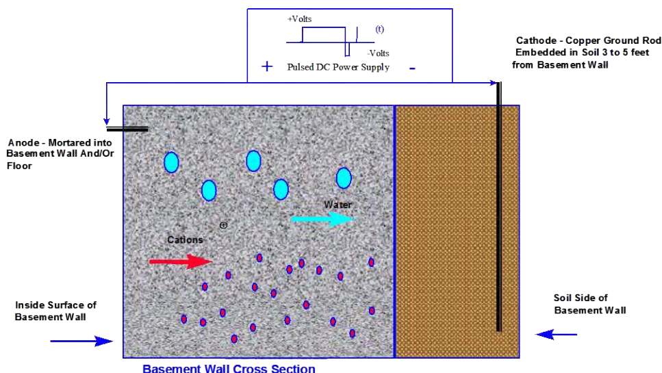
Figure 2.1. Schematic diagram of the EOP system.
