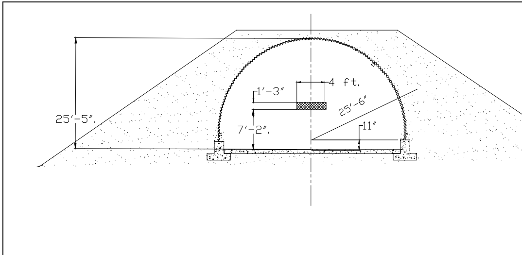
Figure D-6: Area of Maximum Moment on the Back wall.
