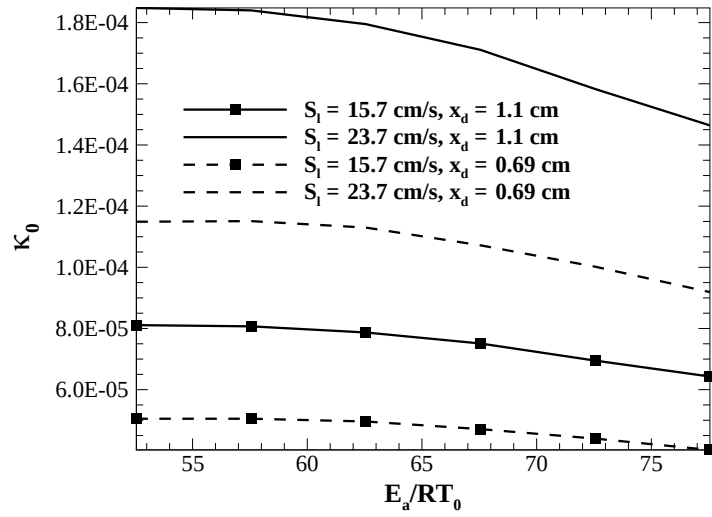
Figure 3.25. Variation of \kappa_o needed to attain S_l = 15.7 or 23.7 \text{ cm/s} using the values of A for which x_d = 0.69 or 1.1 \text{ cm} shown in Figure 3.23b as a function of E_a/RT_0 .
