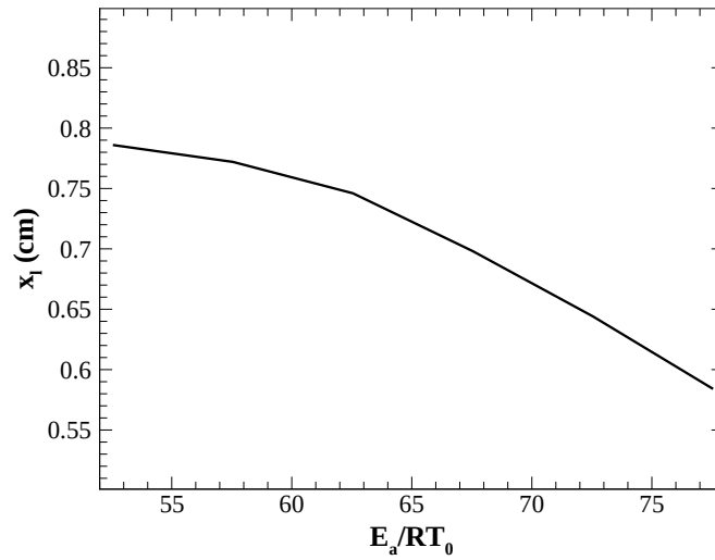
Figure 3.26. Laminar flame thickness computed using values of \kappa_o on the lowest curve in Figure 3.24 ( S_l = 15.7 \text{ cm/s} , x_d = 0.69 \text{ cm} ) as a function of E_a/RT_0 .
