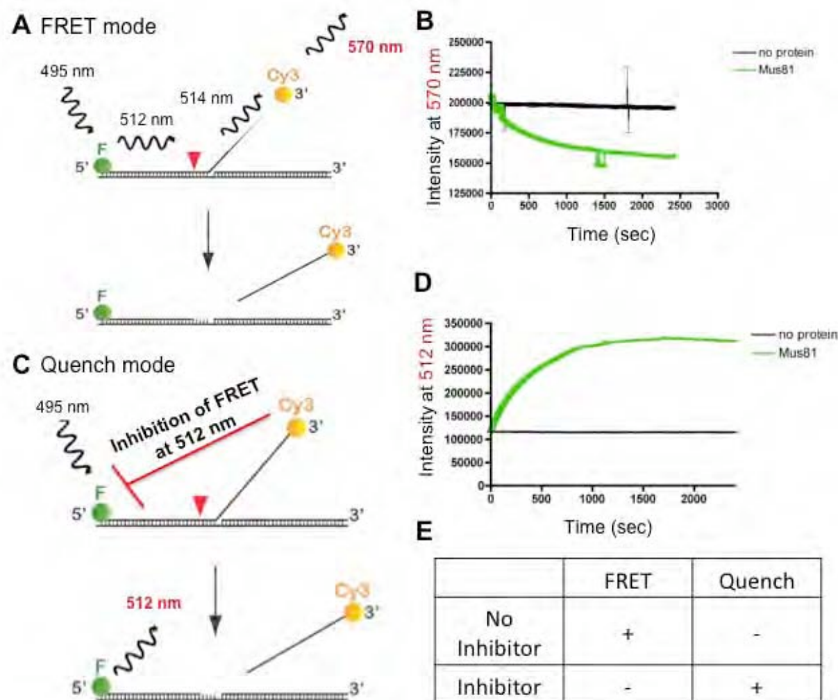
Fig. 3: Fluorescence based nuclease assay in FRET and Quench modes. (A) FRET can be detected by exciting fluorescein (F) ( \lambda_{\text{ex}} = 495 \text{ nm} ) so that it emits a wavelength ( \lambda_{\text{em}} = 512 \text{ nm} ) that is in the same range of excitation wavelength ( \lambda_{\text{ex}} = 514 \text{ nm} ) as Cy3, so Cy3 will emit fluorescence at \lambda_{\text{em}} = 570 \text{ nm} . 570 nm is indicated in red because it is the wavelength at which fluorescence signal is measured in the FRET mode. If HsMUS81-EME1 were to incise a fluorescently labeled substrate (incision point indicated by red triangle) to create a greater distance between the fluorophores, then there will be a loss of FRET signal. (B) Preliminary data showing loss of FRET signal at 570 nm upon addition of 15 nM ScMus81-Mms4 to 25 nM fluorescent DNA substrate. (C) Cy3 is used as a quencher by inhibiting fluorescein emission. Upon HsMUS81-EME1 incision, there will be increase fluorescein emission at \lambda_{\text{em}} = 512 \text{ nm} . 512 nm is indicated in red because it is the wavelength at which fluorescence signal is measured in the Quench mode. (D) Preliminary data showing increase in fluorescein emission at 512 nm upon addition of 15 nM ScMus81-Mms4 to 25 nM fluorescent DNA substrate. (E) Table representing fluorescent signal loss (-) or signal gain (+) in FRET and Quench modes
