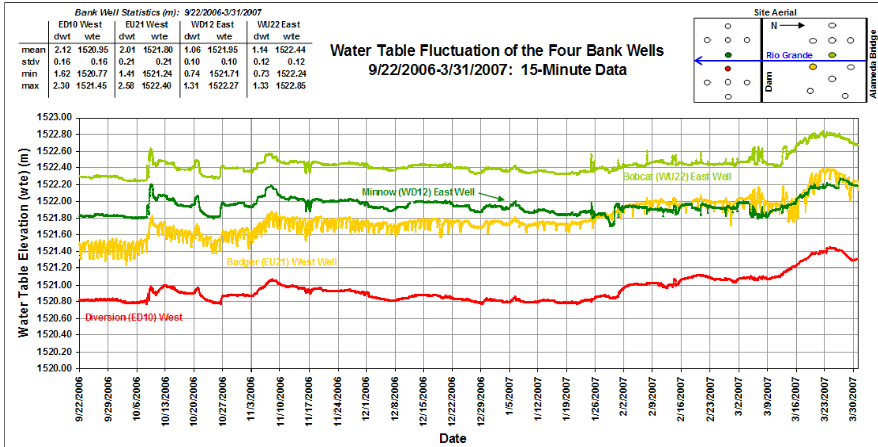
Figure 11. Four bank wells with water table elevation fluctuation.
