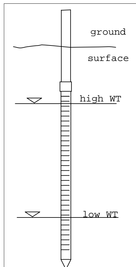
Figure H-1. Intake screen should capture range in WT elevations if possible.
