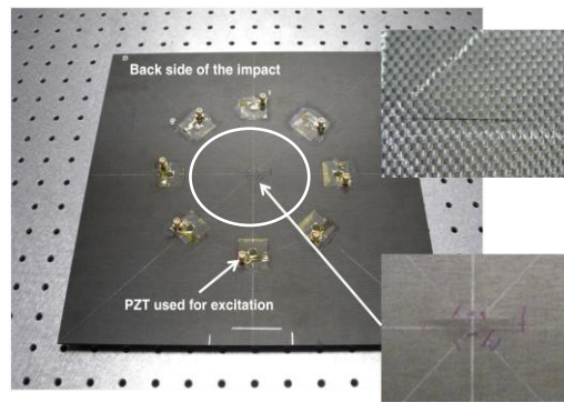
Figure 1: A multi-layer composite plate with impact-induced delamination
