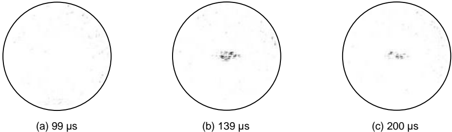
Figure 4: Lamb wave propagation snapshots (with Laplacian filtering)
