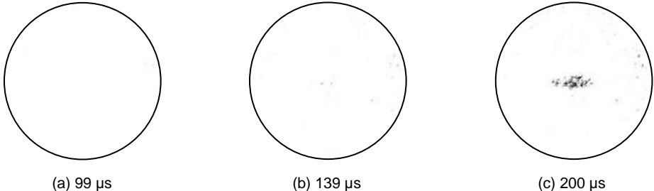
Figure 5: Cumulative kinetic energy evolution snapshots (with Laplacian filtering)
