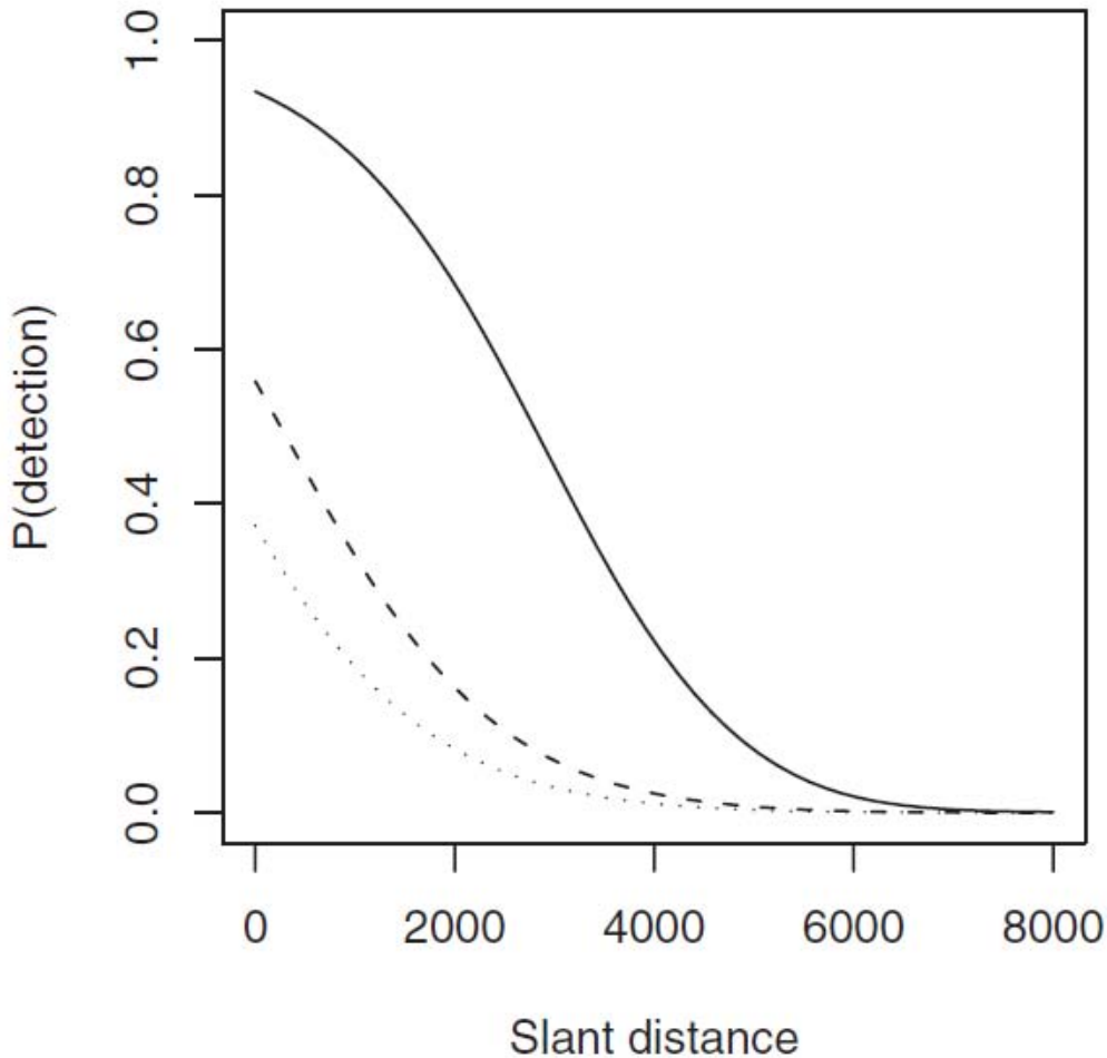
Figure 8. The estimated detection function for Mesoplodon densirostris echolocation clicks detected at AUTEK. The off-axis angles are fixed at 0, 45, and 90° respectively by the solid, dashed, and dotted lines. Figure reproduced from Marques et al. 2009.
