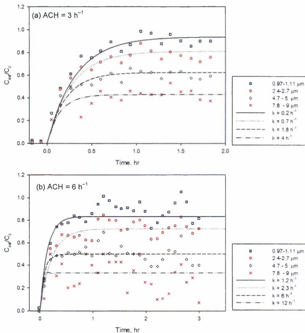
Figure 8. Comparison of modeling calculations with laboratory data in the SST particle infiltration experiments under two different ACH settings. The values of ACH were obtained using \text{CO}_2 tracer gas decay method.
