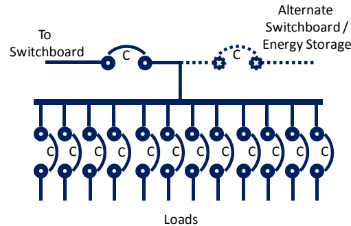
Figure 6. Control centric Load Center topology for implementing QOS and Mission Priority Load Shedding
