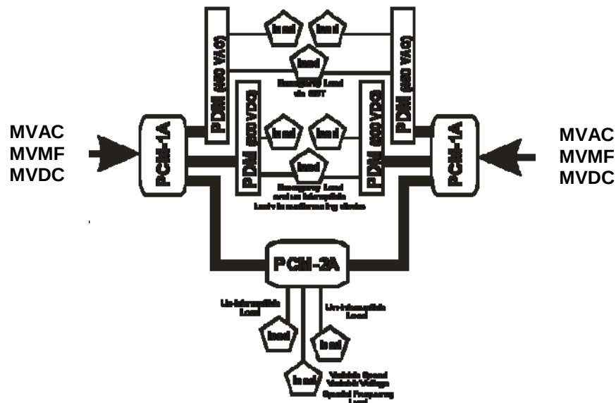
Figure 2. Zonal Electrical Distribution Architecture [5]
