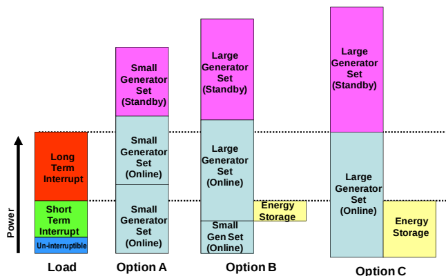
Figure 4. Generator and Energy Storage Sizing
