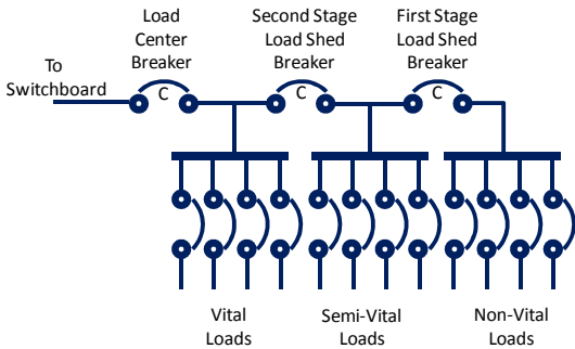
Figure 5. Traditional Load Shedding Implementation in a Load Center
