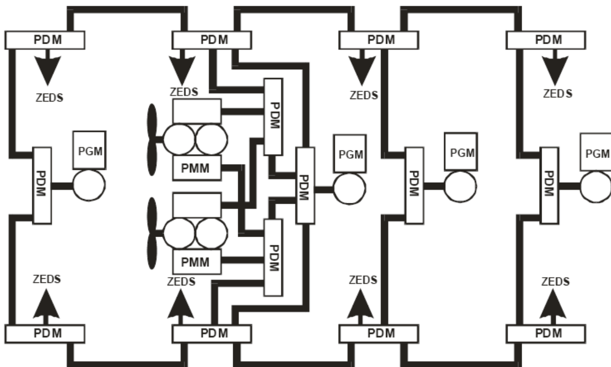
Figure 1. Power Generation Architecture [5]
