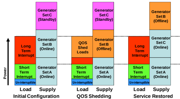
Figure 7. Quality of Service Load Shedding and Restoration of Power
