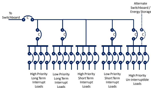
Figure 9. Traditional Load Center implementation modified for QOS
