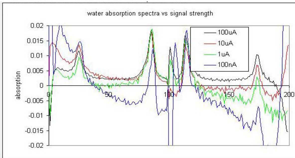
Figure 33: absorption spectra vs detected signal strength
