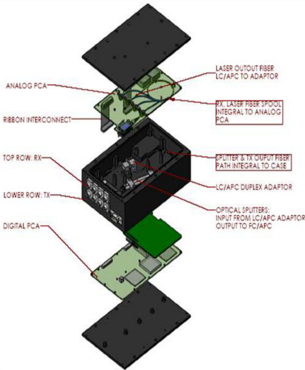
Figure 15: exploded view
