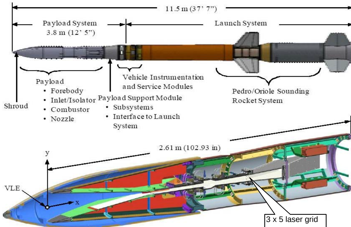
Figure 53: HIFiRE Flight 2.
