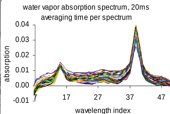
Figure 35: 100 absorption spectra
