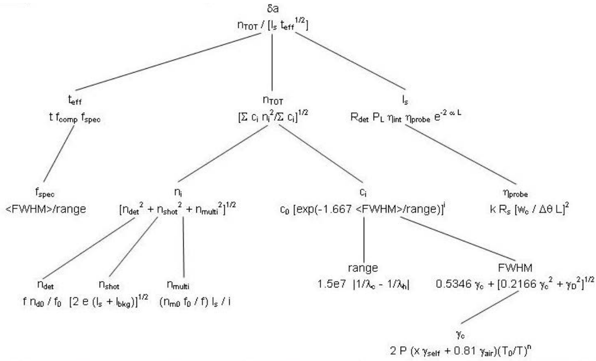
Figure 8: Contributions to light absorption uncertainty
