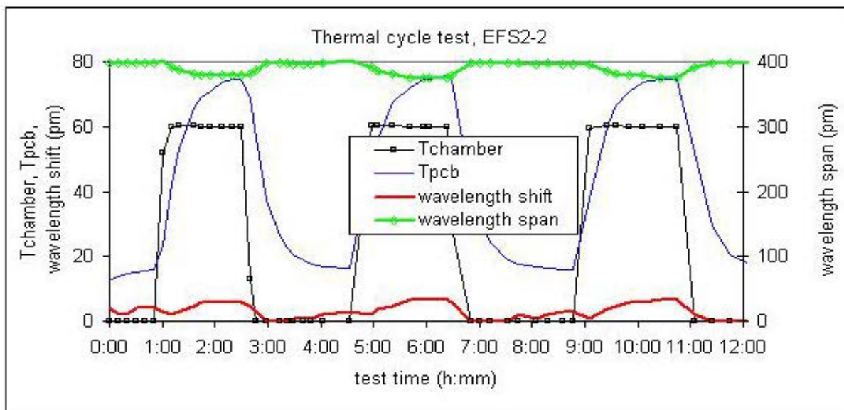
Figure 38: laser wavelength stability with digital temperature control
