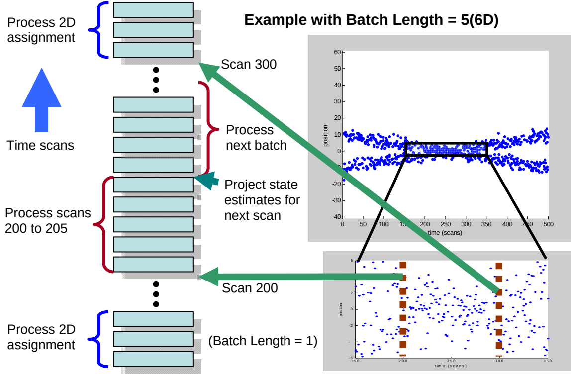
Figure 6. Example of 6D assignment for two-target case with 500 scans and target crossings for 100 scans.
