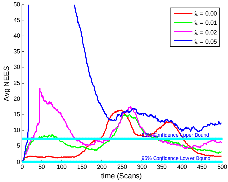
Figure 28. Average NEES for Algorithm II: 2D-4D LP, \sigma_q = 0.002 .
