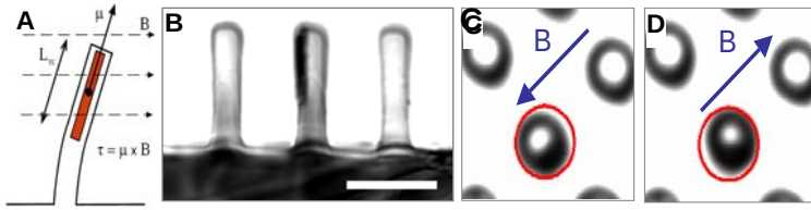
Figure 2. Schematic of piezomagnetic torque of a nanowire in a PDMS post (A). Cross-sectional optical micrograph showing a nanowire embedded in a PDMS post (B, bar: 10 \mu m). Image frames taken from a video show magnetic actuation of a nanowire post at (C) B = -0.2 T. (D) B = +0.2 T. Red circles are
