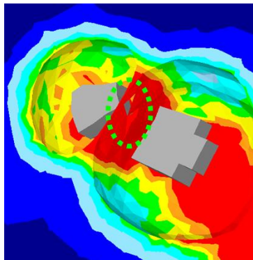
Figure 31: Detail of the initiation of coalescence of voids growing around a pair of particles. (Dotted green line highlights separation of ligament between pores).
