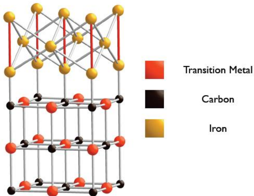
Figure 25: Structure of an iron carbide interface.
