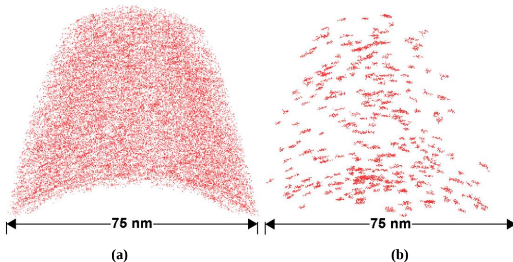
Figure 7: (a) Cu atoms and (b) Cu precipitates in a sample aged for 5 min at 450 °C. Datasets (a) and (b) contain 7 M and 60,000 atoms, respectively.
