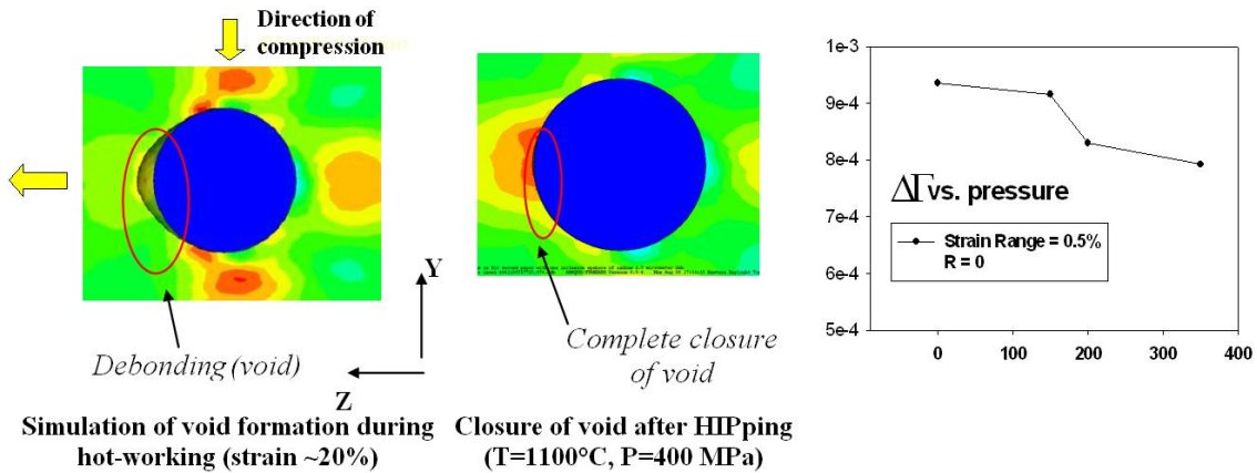
Figure 17: Assessment of Hot Isostatic Pressing (HIPping) on healing of process damage and enhancement of fatigue performance of gear steels.
