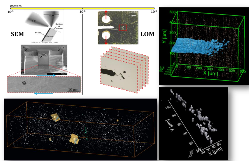
Figure 1: Development of experimental techniques and analysis/visualization tools for SEM and LOM level 3D microstructure, including precipitates, inclusions, hot working damage, microvoids and ductile fracture process
