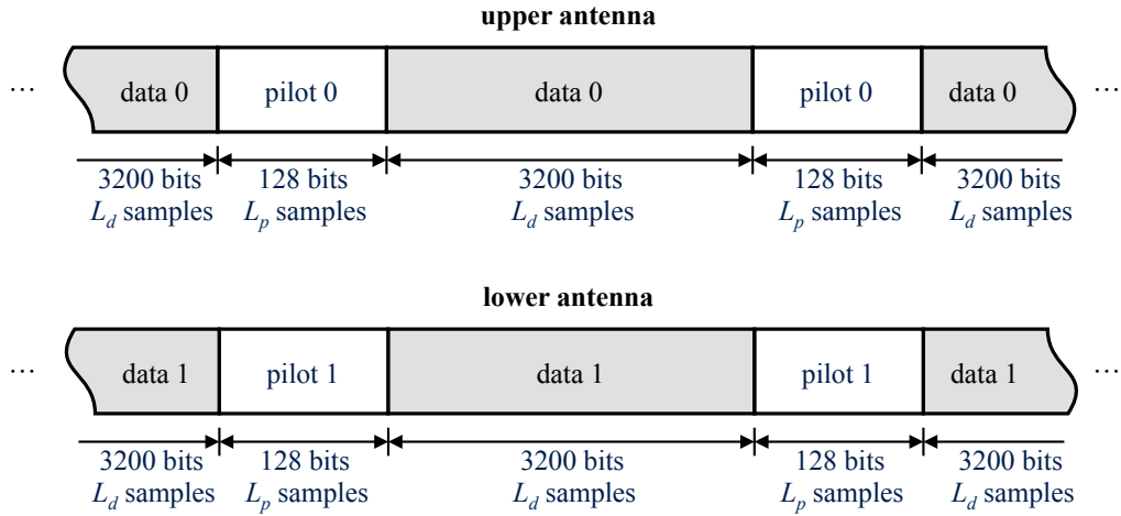
Figure 3: The relationship between the data and pilot bits used for the space-time coded system.
