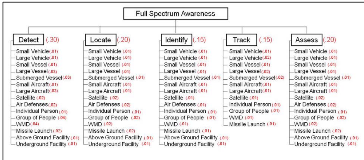
Figure 31. Condensed Hierarchy with Hypothetical Global Weights
