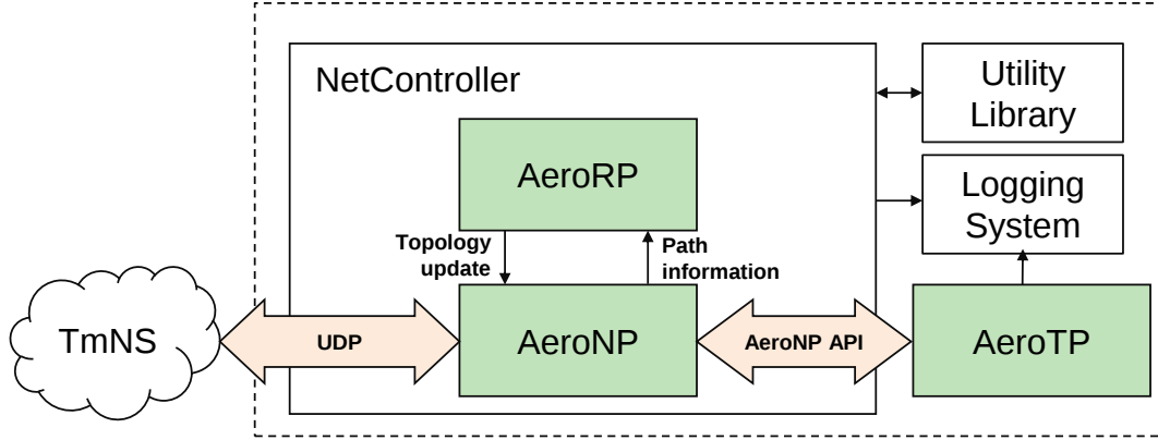
Figure 1: System Architecture
