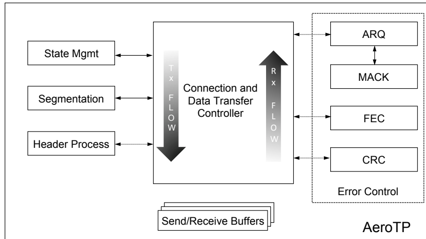
Figure 2: AeroTP implementation architecture
