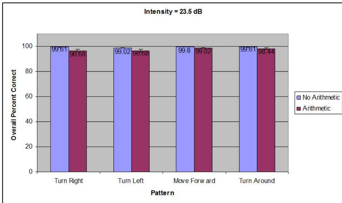
Figure 11. Intensity (23.5 dB) \times Pattern \times Arithmetic interaction (overall percent correct).
