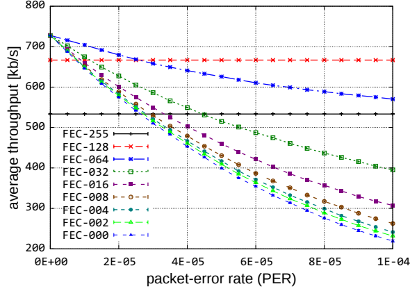
Figure 5: Average goodput
