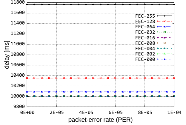
Figure 6: Average delay
