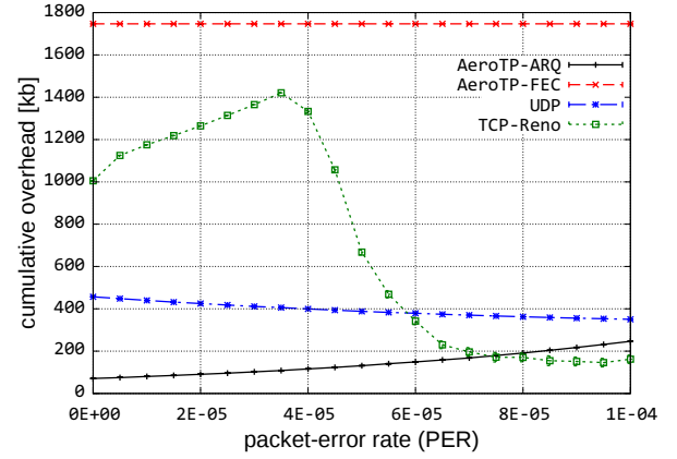
Figure 16: Cumulative overhead
