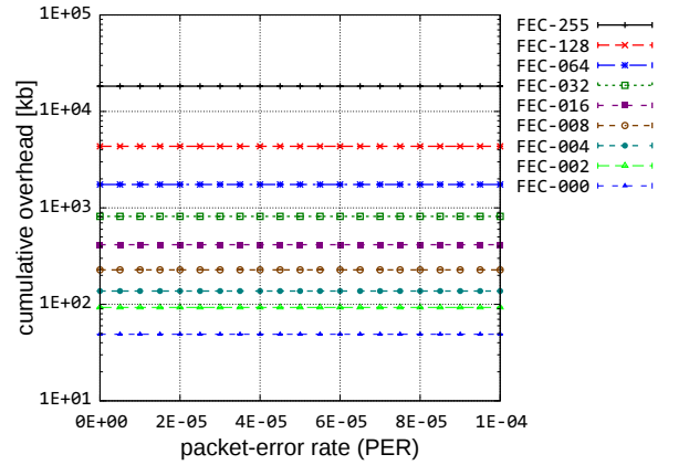
Figure 8: Cumulative overhead
