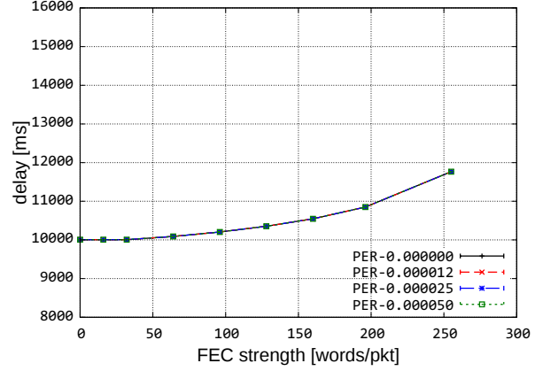
Figure 10: Average delay
