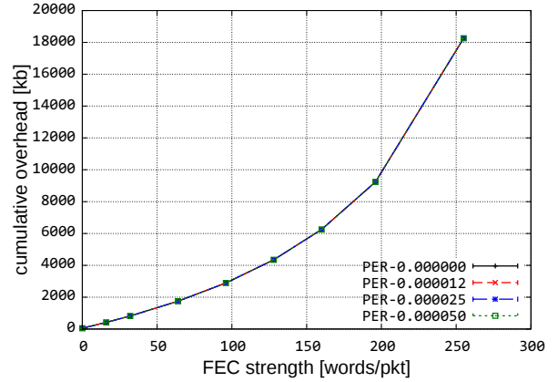
Figure 12: Cumulative overhead
