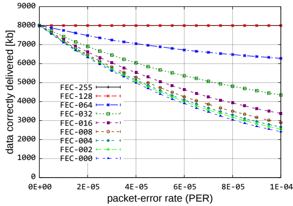
Figure 7: Cumulative goodput
