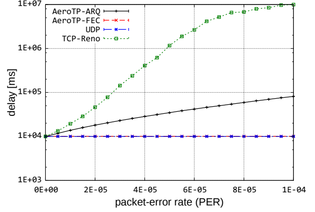
Figure 14: Average delay
