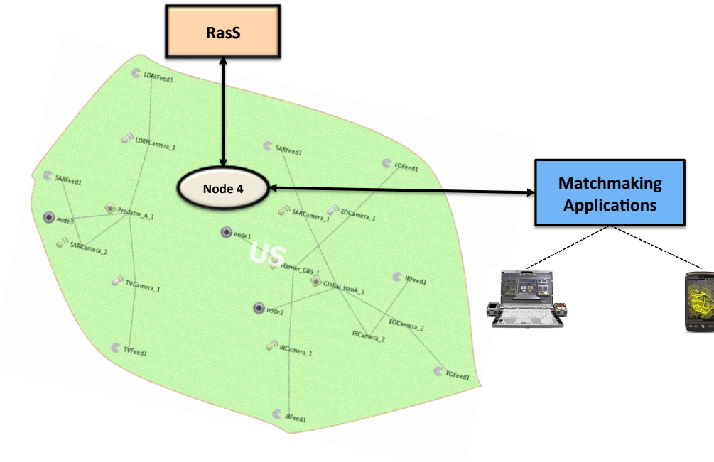
Figure 4. Resource-Task Assignment Application based on RasS
