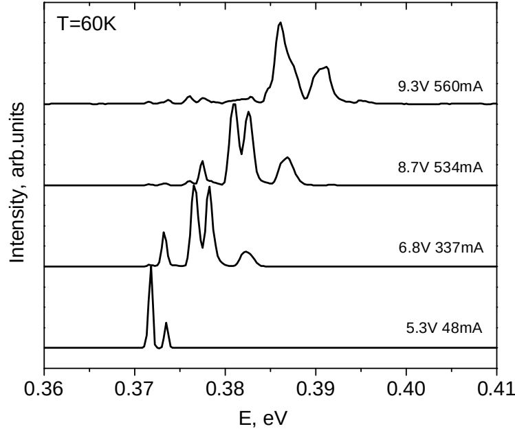
Figure 7 Lasing spectra of the tunable IC laser at different values of the injection current.
