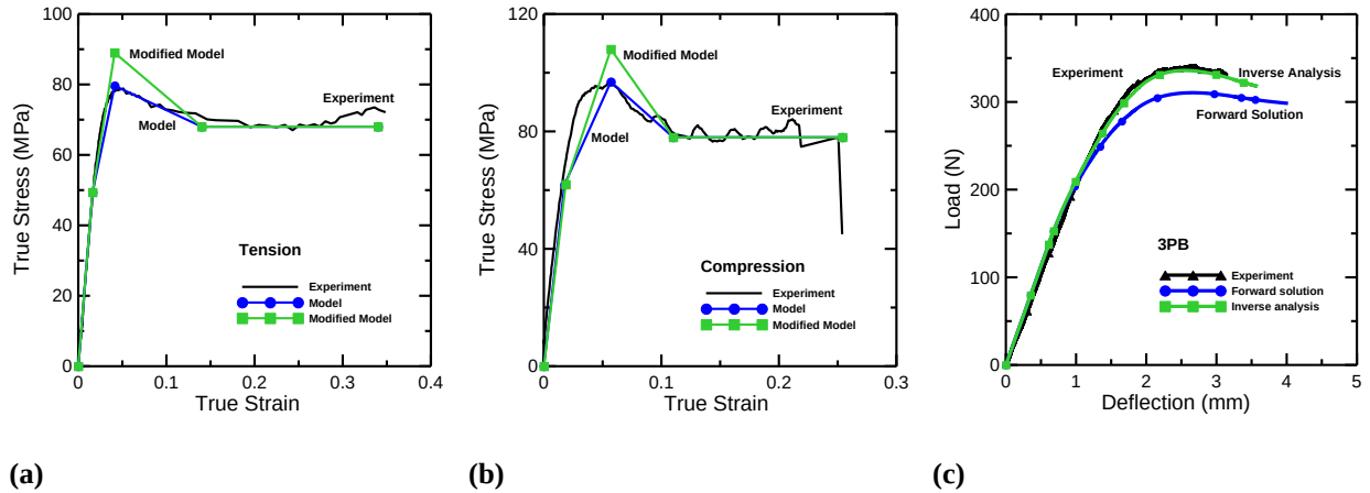
Fig. 12 Experiment and simulation of tension, compression and load deflection response at 493 \mu str/sec
