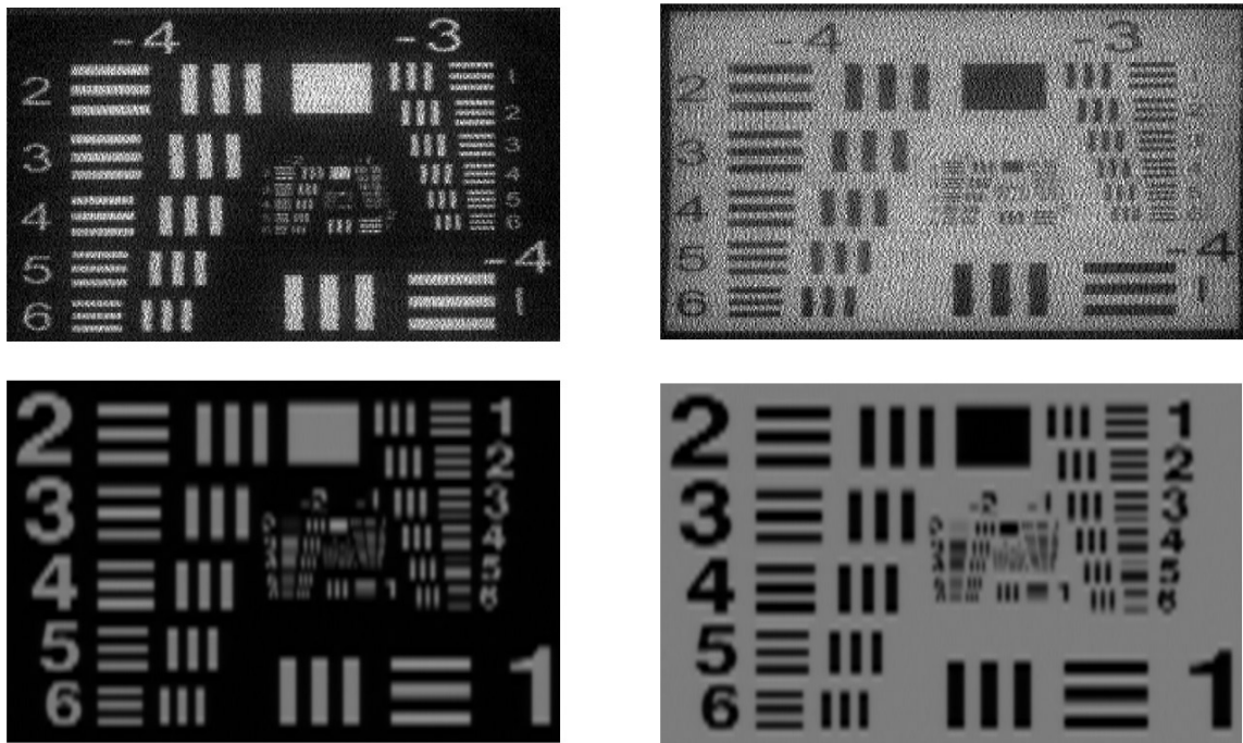
Figure 5: Raw images (top) and simulated images (bottom) of USAF technical targets at 2.2 attenuation lengths. [Polygon speed = 1000rpm, stand-off distance = 5m, b=0.29m^{-1} , c=0.43m^{-1} ]
