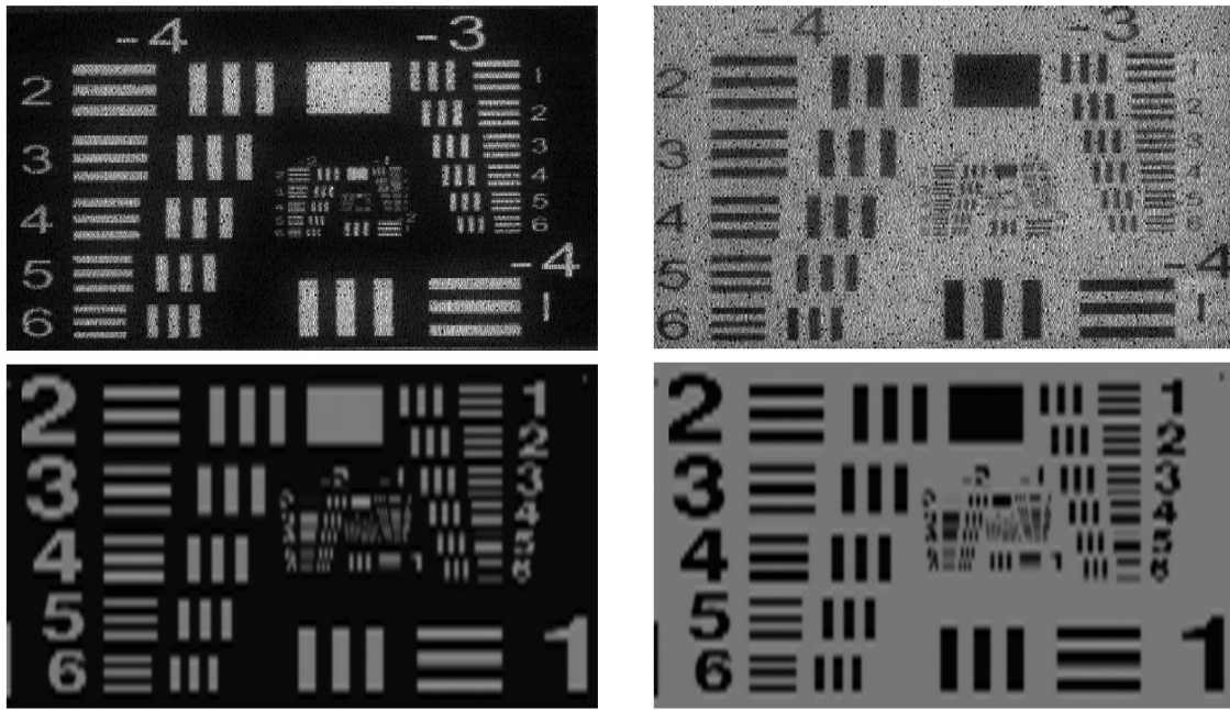
Figure 4: Raw images (top) and simulated images (bottom) of USAF technical targets at 1.3 attenuation lengths. [Polygon speed = 1000rpm, stand-off distance = 3m, b=0.29m^{-1} , c=0.43m^{-1} ]
