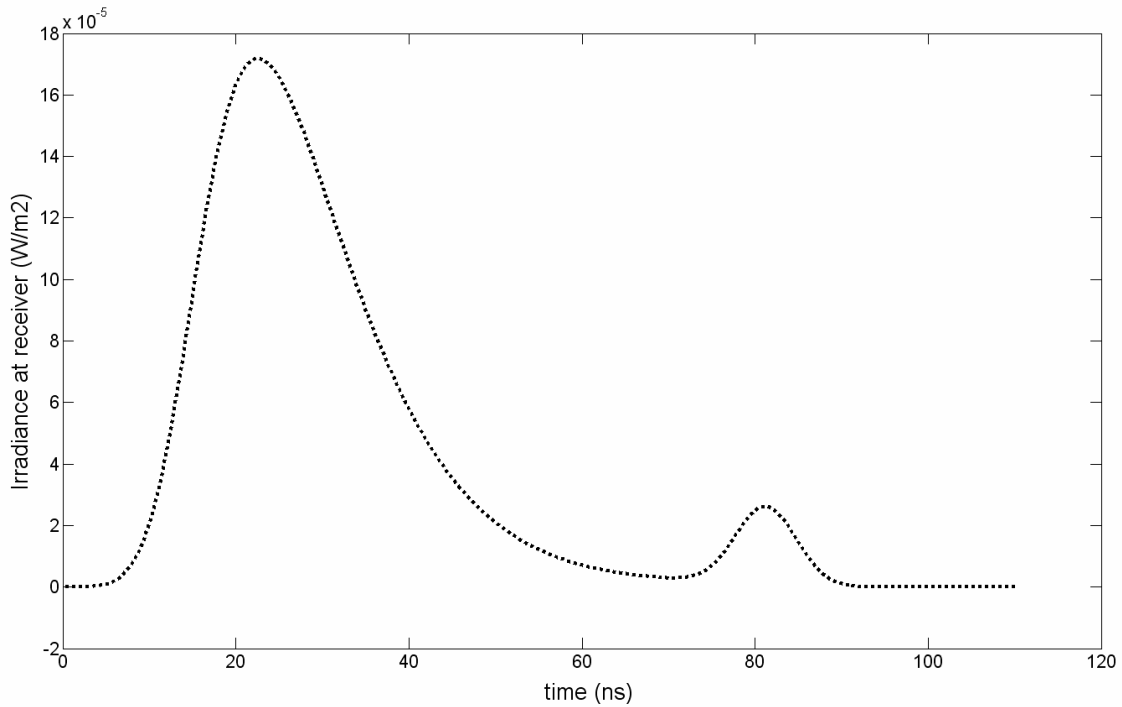
Figure 1: Temporal return at receiver for highly scattering coastal waters ( b=0.9m^{-1} , c=1.0m^{-1} ) at 9 attenuation lengths (9 meters). [Laser pulse FWHM = 7ns. Average power at 350KHz = 2.5W. Source-receiver separation = 0.1m. Angular aperture = 15mrad. Target reflectance = 0.1. McLean-Freeman phase function is used.]
